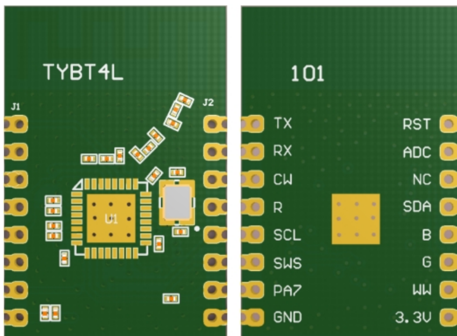
Figure 2.1 TYBT4L footprint
