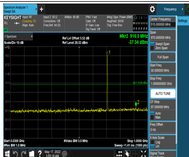
Band12-1.4MHz-16QAM-23173-1RB#0-Range3:30~1000MHz
