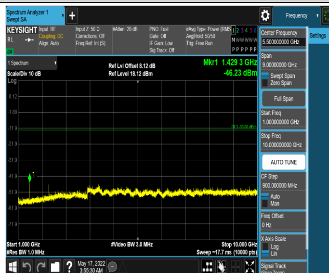
Band12-1.4MHz-16QAM-23173-1RB#0-Range4:1000~10000MHz
