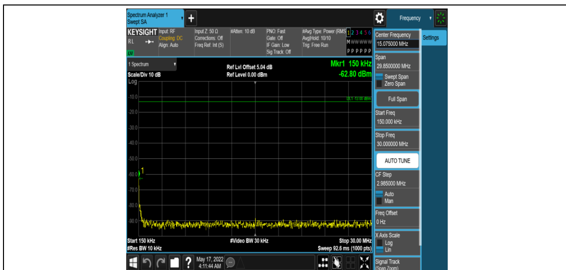
Band12-3MHz-16QAM-23025-1RB#0-Range2:0.15~30MHz
