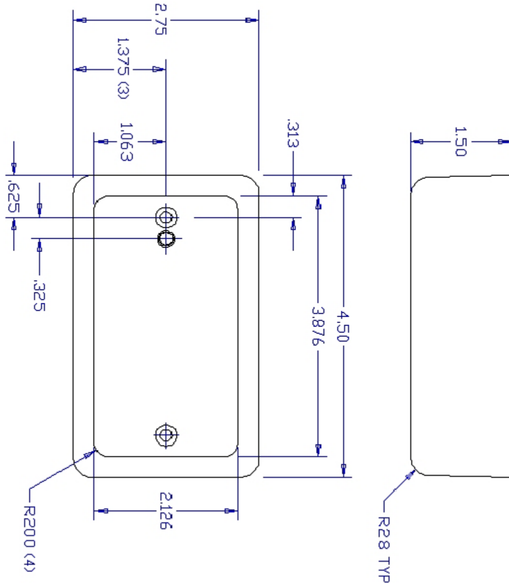
Figure 3. GO CARD Access Control Target, Small
