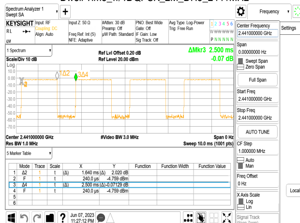
Dwell Time_π/4DQPSK_2M_DH5_2441MHz
