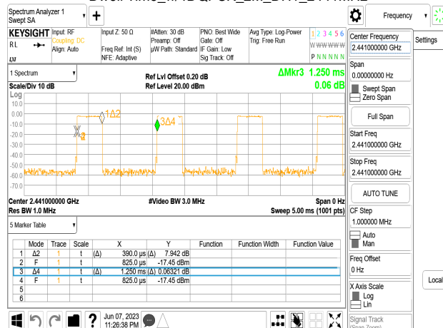
Dwell Time_π/4DQPSK_2M_DH3_2441MHz
