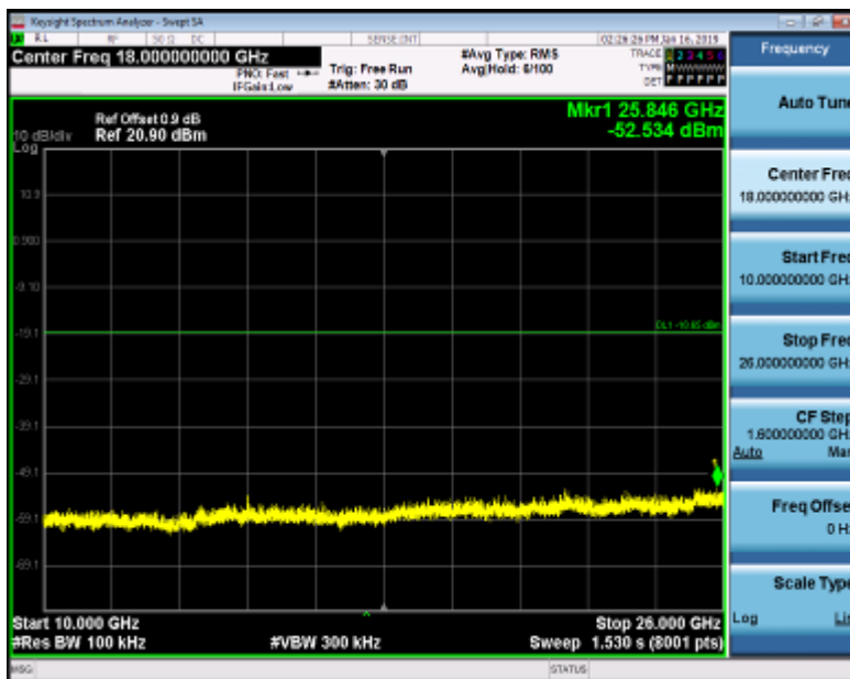
RF Conducted Spurious Emissions_11N40SISO_2422_Ant1
