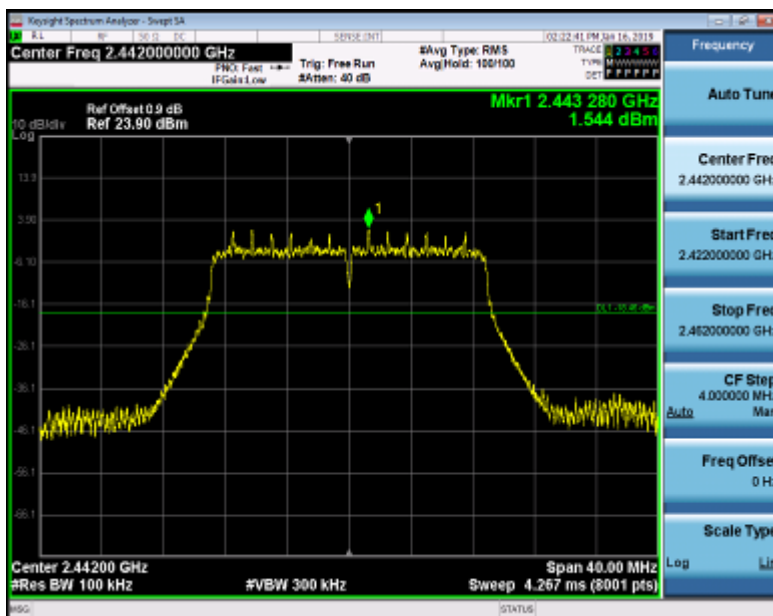
RF Conducted Spurious Emissions_11N20SISO_2442_Ant1
