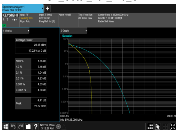
N25(20M)_DFT-s-OFDM_PI_2-BPSK_Outer_Full_Mid_CH
