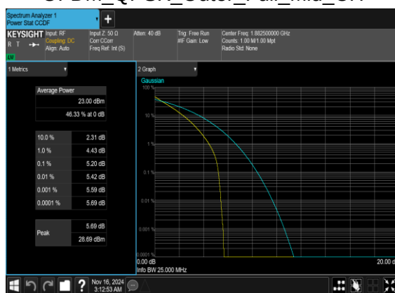
N25(20M)_DFT-s-OFDM_QPSK_Outer_Full_Mid_CH
