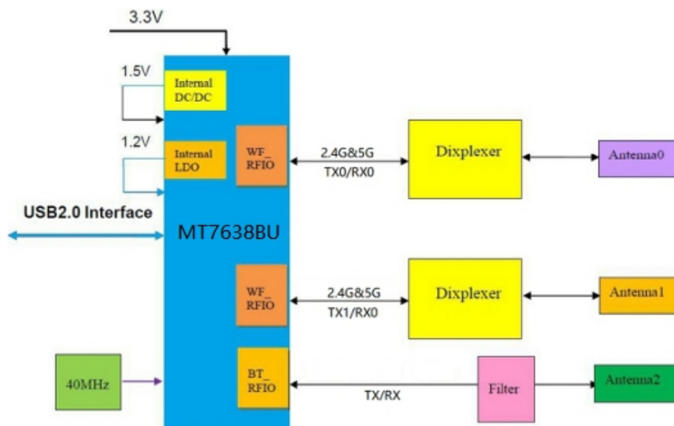
Figure 1 EL.MT7638BUN-WF Block Diagram
