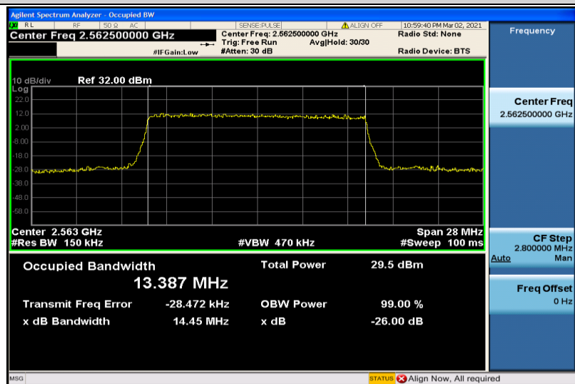
Band7-15MHz-16QAM-21375-75RB#0-13.387
