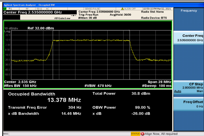
Band7-15MHz-QPSK-21100-75RB#0-13.378
