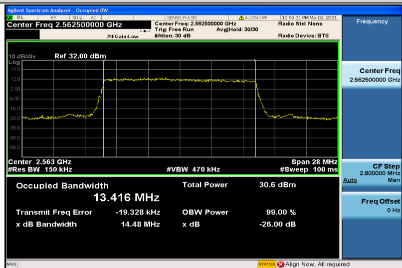
Band7-15MHz-QPSK-21375-75RB#0-13.416
