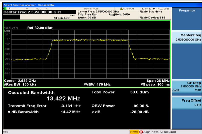
Band7-15MHz-16QAM-21100-75RB#0-13.422
