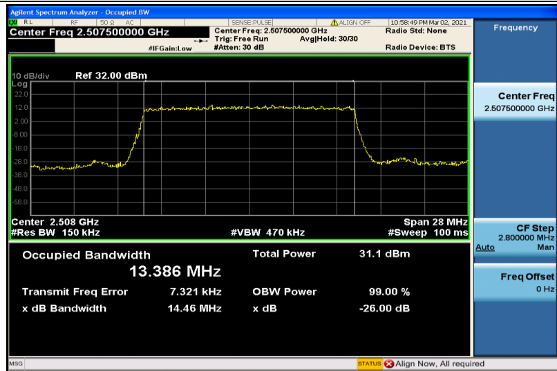
Band7-15MHz-QPSK-20825-75RB#0-13.386
