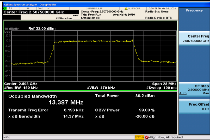
Band7-15MHz-16QAM-20825-75RB#0-13.387
