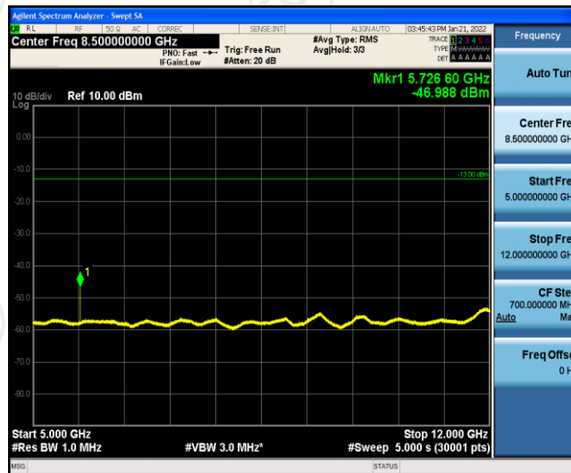
Band2-1.4MHz-QPSK-19193-1RB#0-Range6:12000~26500MHz
