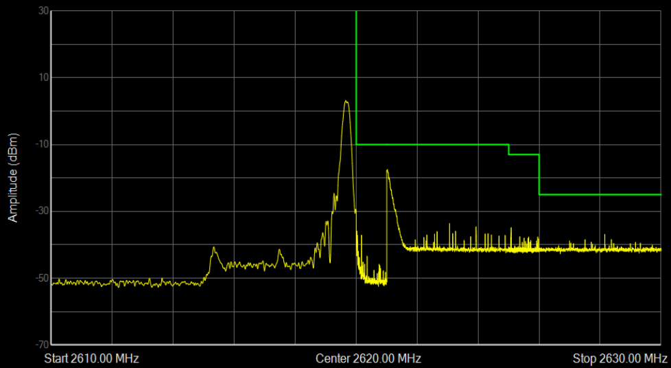
Band41 16QAM BW=5MHz Channel=40865 RB Size=1 Position=#Max
