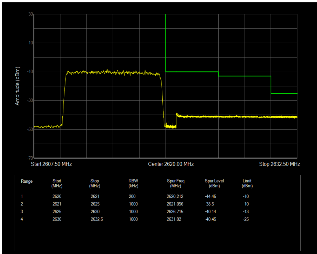
Band41 16QAM BW=10MHz Channel=40840 RB Size=1 Position=#0
