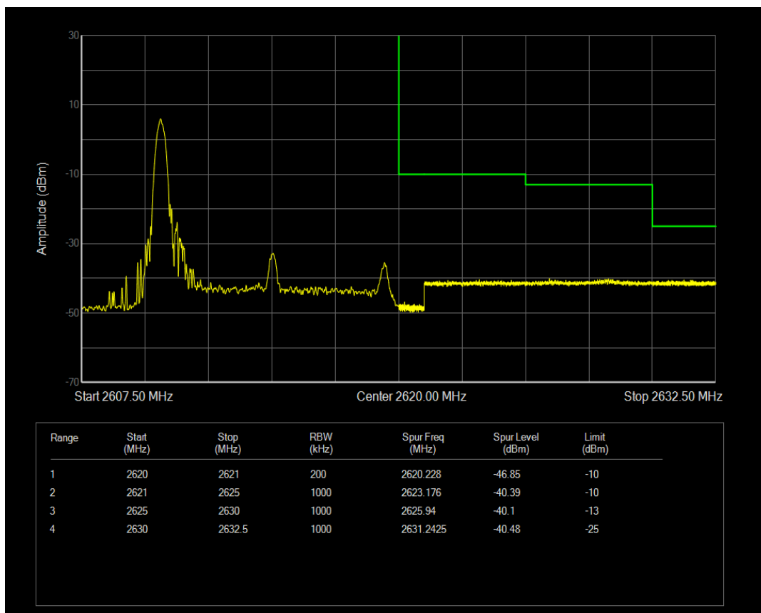
Band41 QPSK BW=10MHz Channel=40840 RB Size=1 Position=#Max
