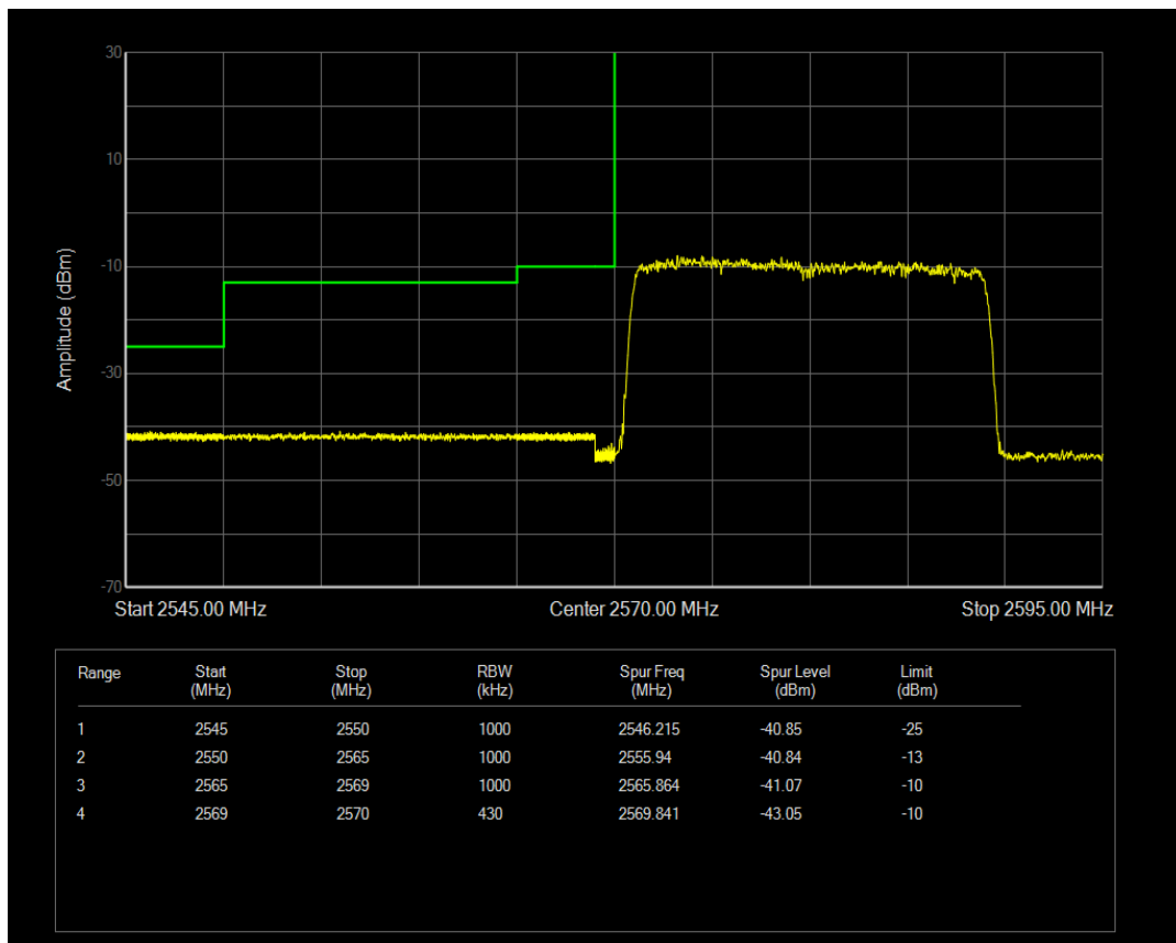
Band41 16QAM BW=20MHz Channel=40490 RB Size=1 Position=#0
