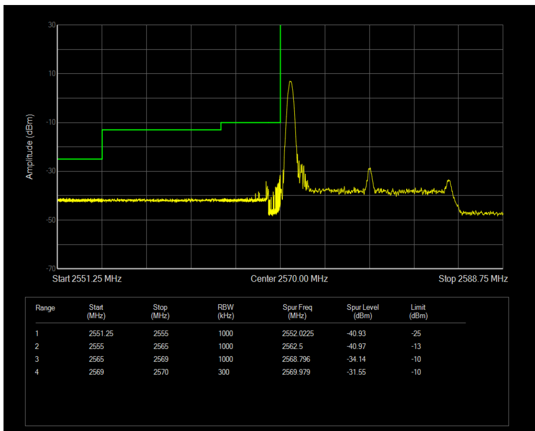
Band41 QPSK BW=15MHz Channel=40465 RB Size=1 Position=#Max
