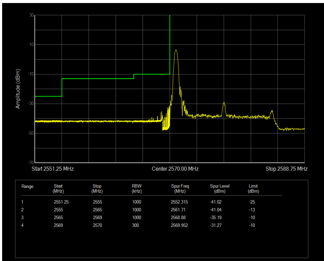
Band41 16QAM BW=15MHz Channel=40465 RB Size=1 Position=#Max
