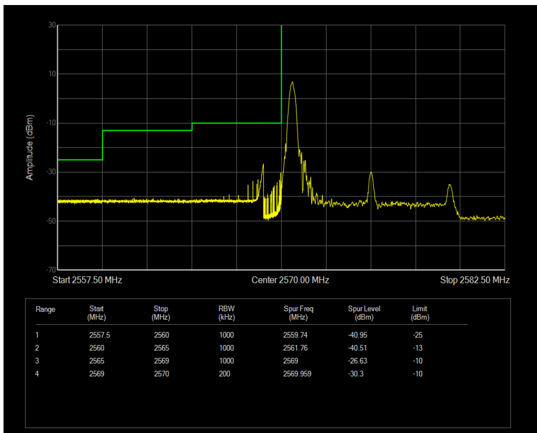
Band41 QPSK BW=10MHz Channel=40440 RB Size=1 Position=#Max
