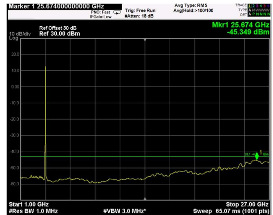
Channel: TOP, Modulation: 256QAM, BW=5MHz, Range: 1GHz - 27GHz
