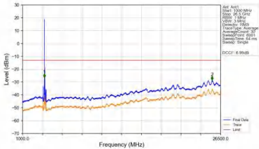
n77a_30kHz_SISO_NTNV_80MHz_DFT-s-OFDM_QPSK_3840MHz_Edge_1RB_Left_Ant1
