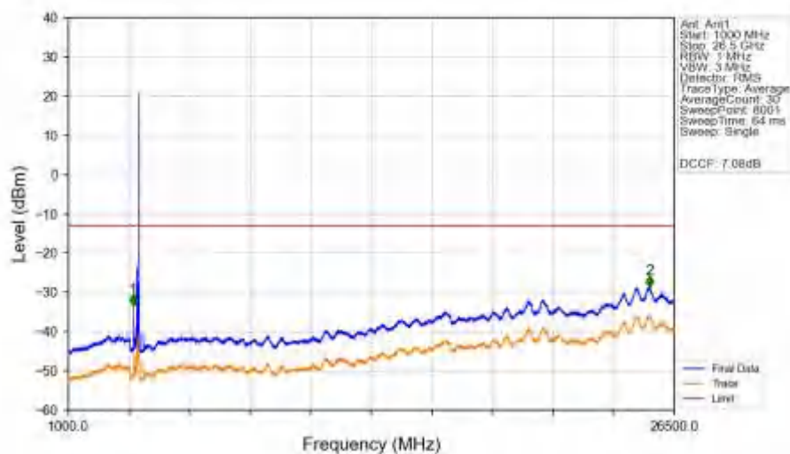
n77a_30kHz_SISO_NTNV_90MHz_CP-OFDM_QPSK_3934.98MHz_Edge_1RB_Right_Ant1
