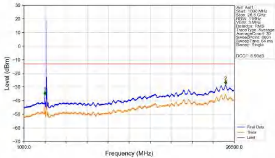
n77a_30kHz_SISO_NTNV_90MHz_CP-OFDM_QPSK_3745.02MHz_Edge_1RB_Left_Ant1
