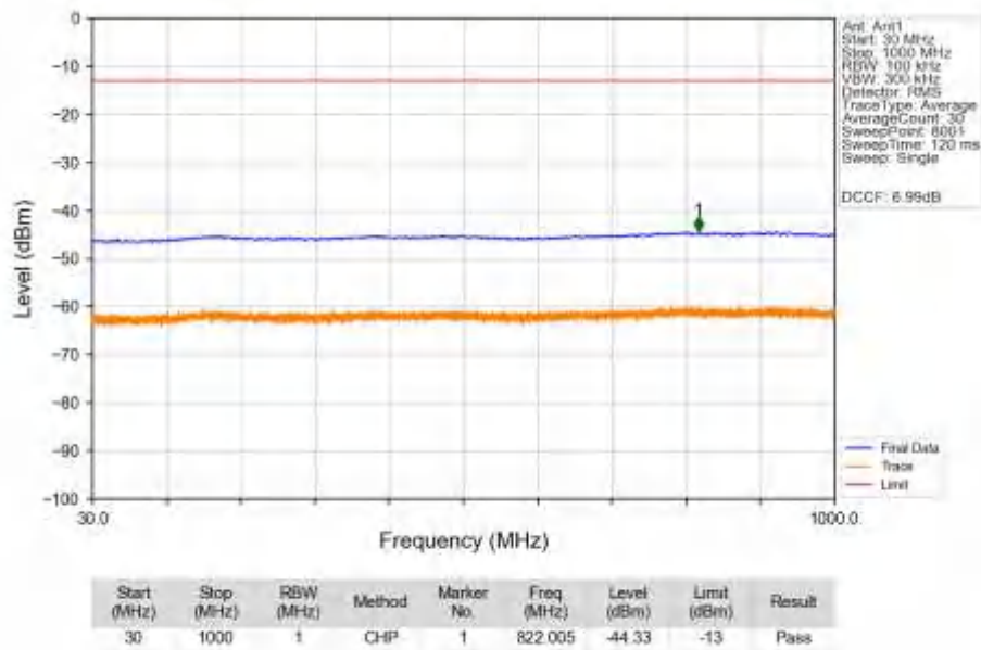
n77a_30kHz_SISO_NTNV_100MHz_DFT-s-OFDM QPSK_3750MHz_Edge_1RB_Left_Ant1
