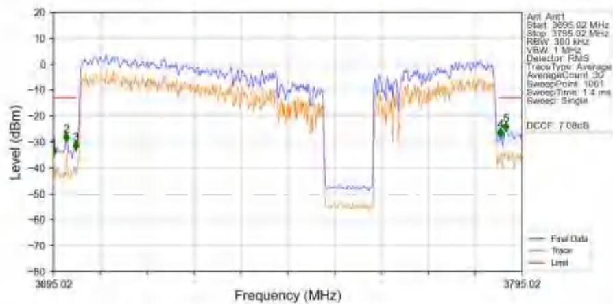
n77a_30kHz_SISO_NTNV_90MHz_CP-OFDM_QPSK_3745.02MHz_Outer_Full_Ant1
