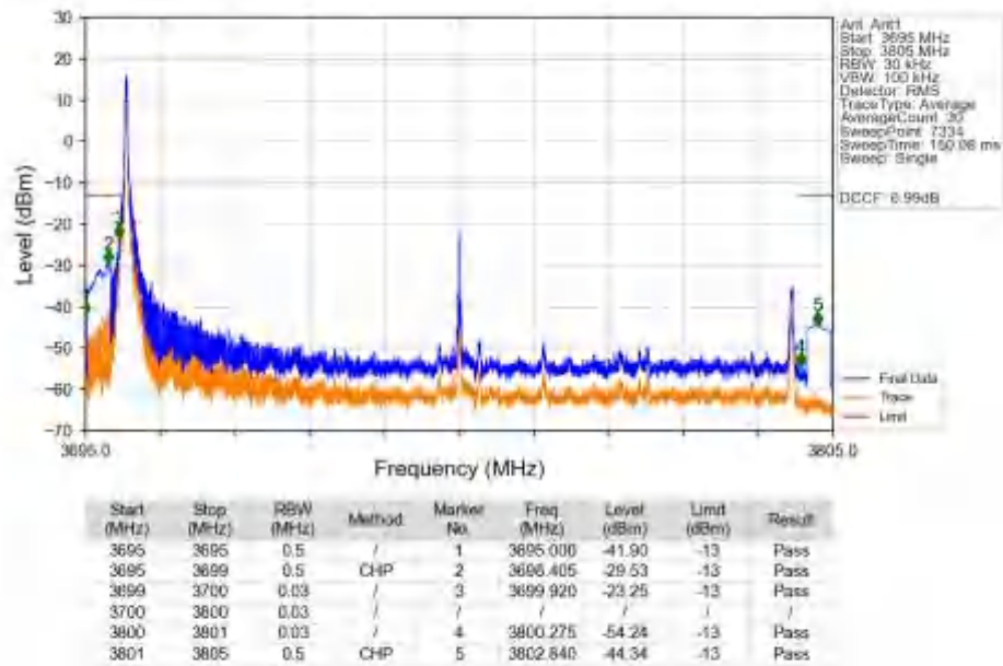
n77a_30kHz_SISO_NTNV_100MHz_DFT-s-OFDM QPSK_3750MHz_Edge_1RB_Left_Ant1
