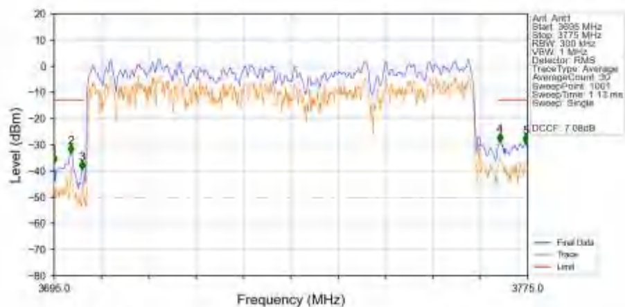
n77a_30kHz_SISO_NTNV_70MHz_DFT-s-OFDM_QPSK_3735MHz_Outer_Full_Ant1
