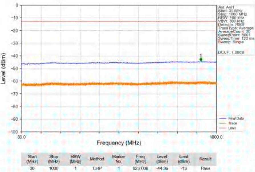
n77a_30kHz_SISO_NTNV_70MHz_CP-OFDM_QPSK_3840MHz_Edge_1RB_Left_Ant1
