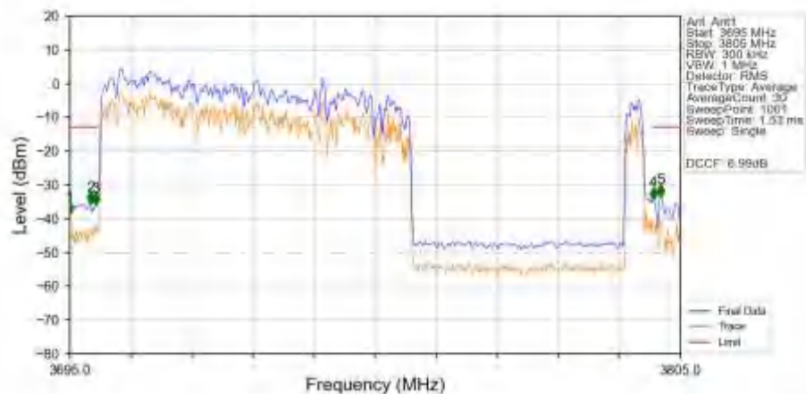
n77a_30kHz_SISO_NTNV_100MHz_DFT-s-OFDM_QPSK_3750MHz_Outer_Full_Ant1
