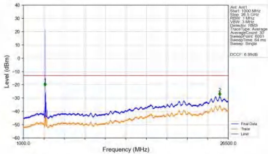
n77a_30kHz_SISO_NTNV_70MHz_DFT-s-OFDM_QPSK_3735MHz_Edge_1RB_Left_Ant1
