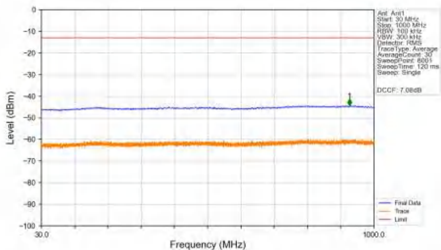
n77a_30kHz_SISO_NTNV_90MHz_CP-OFDM_QPSK_3934.98MHz_Edge_1RB_Right_Ant1
