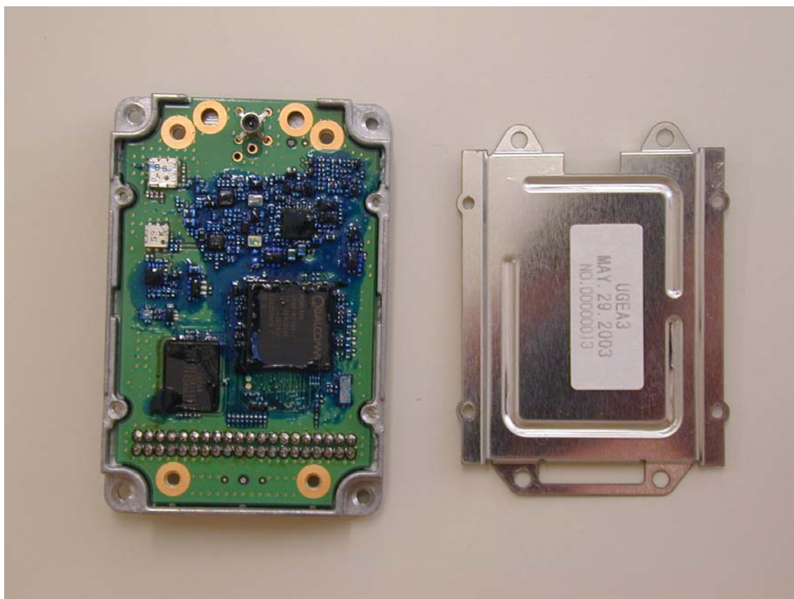
Cover opened (Back side)
