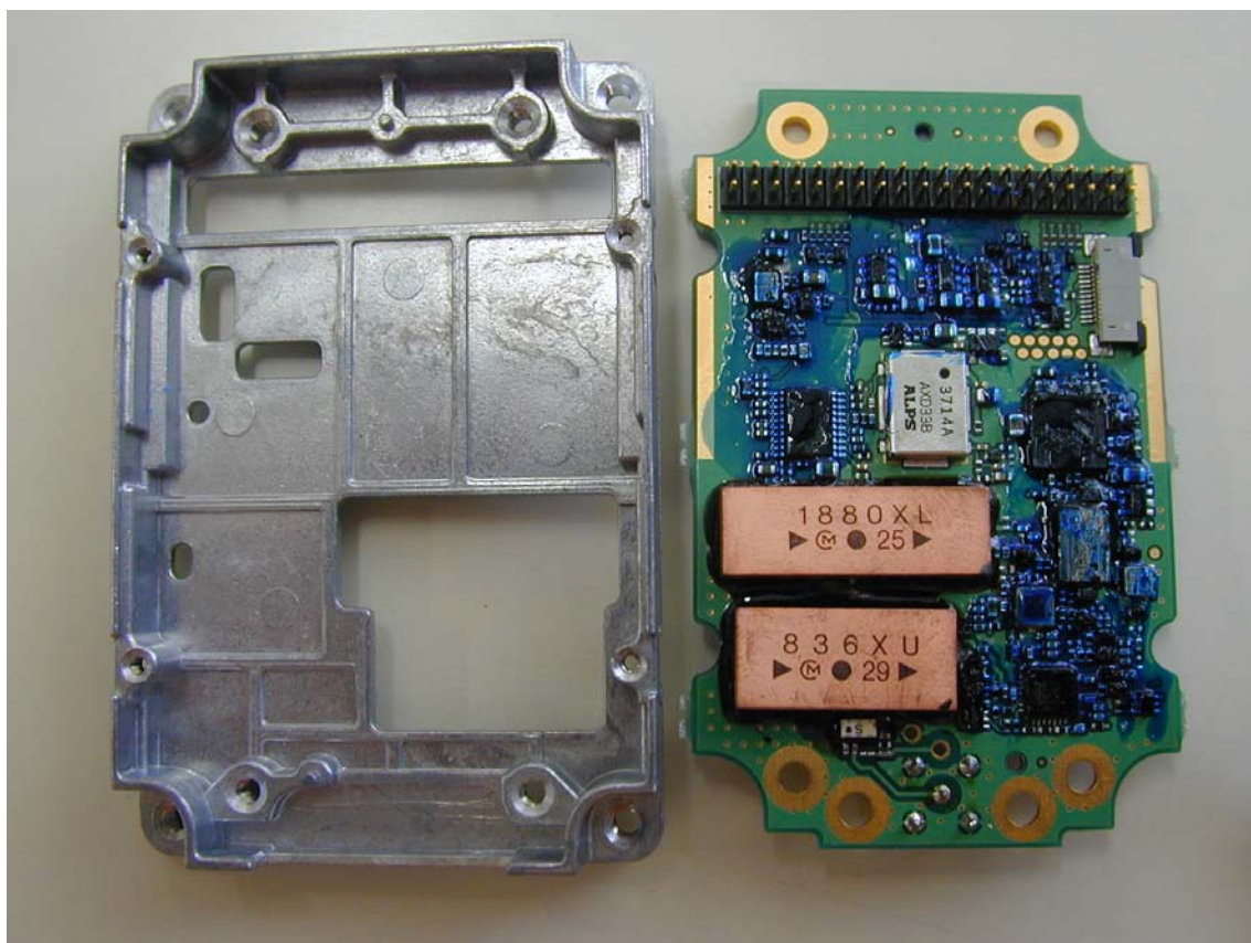
Cover opened (Front side)
