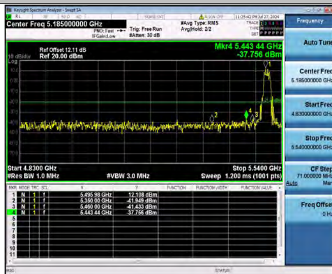
11N20SISO_Ant1_Low_5500_AV
