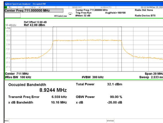
Band 12 10MHz/711.0/High 16QAM 50@0
