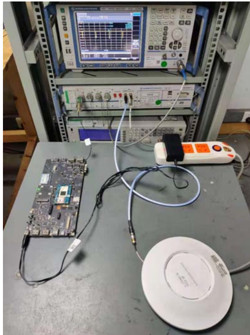
DFS setup photo
