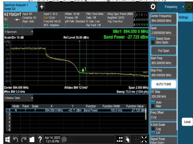
Plot 8-280. Band Edge Emission Summary Data Plot (LTE B5_1C_10M_256QAM - High Channel_2T, Port 1)
