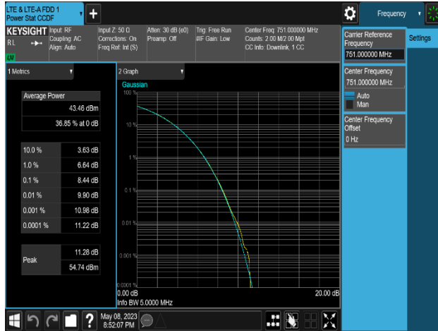
Plot 8-269. Peak To Average Power Ratio Plot (LTE B13_1C_5M_QPSK - Mid Channel_4T, Port 0)
