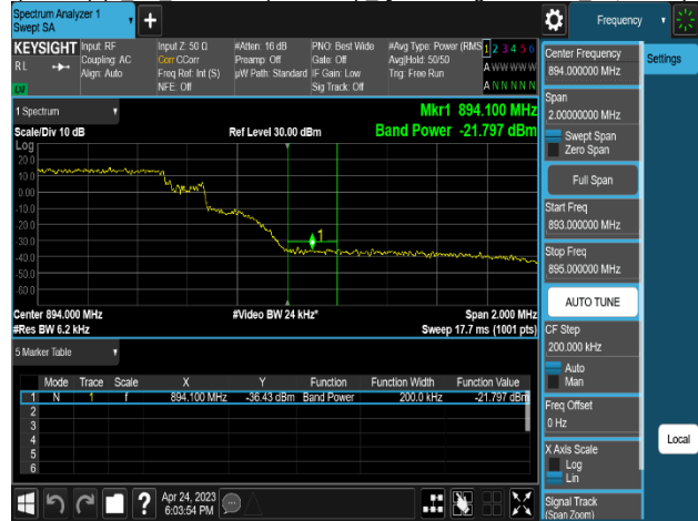
Plot 8-306. Band Edge Emission Summary Data Plot (DSS B(n)5_2NC_10M+10M(9:1 Ratio)_QPSK - High Channel 2T, Port 1)
