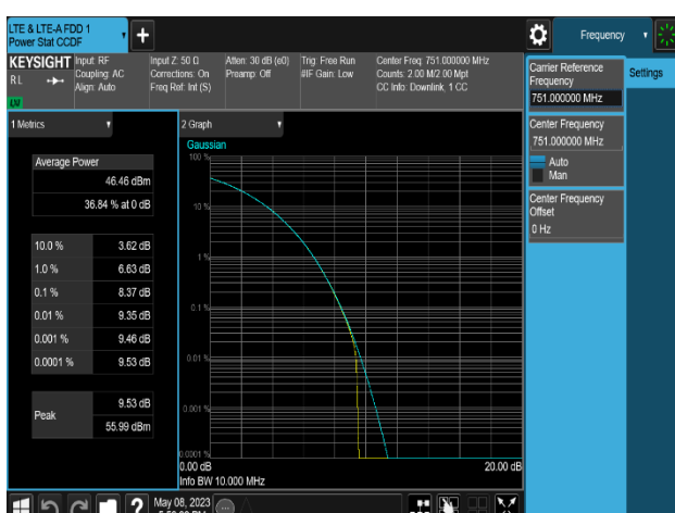
Plot 8-271. Peak To Average Power Ratio Plot (LTE B13_1C_10M_QPSK - Mid Channel_4T, Port 0)
