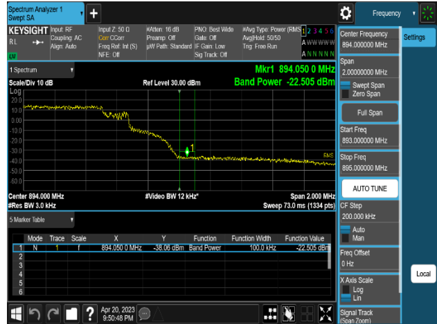
Plot 8-290. Band Edge Emission Summary Data Plot (DSS B(n)5_1C_10M(8:2 Ratio)_256QAM - High Channel 2T, Port 1)
