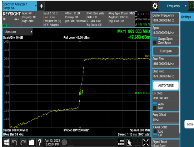
Plot 8-277. Band Edge Emission Summary Data Plot (LTE B5_1C_5M_64QAM - Low Channel_2T, Port 0)
