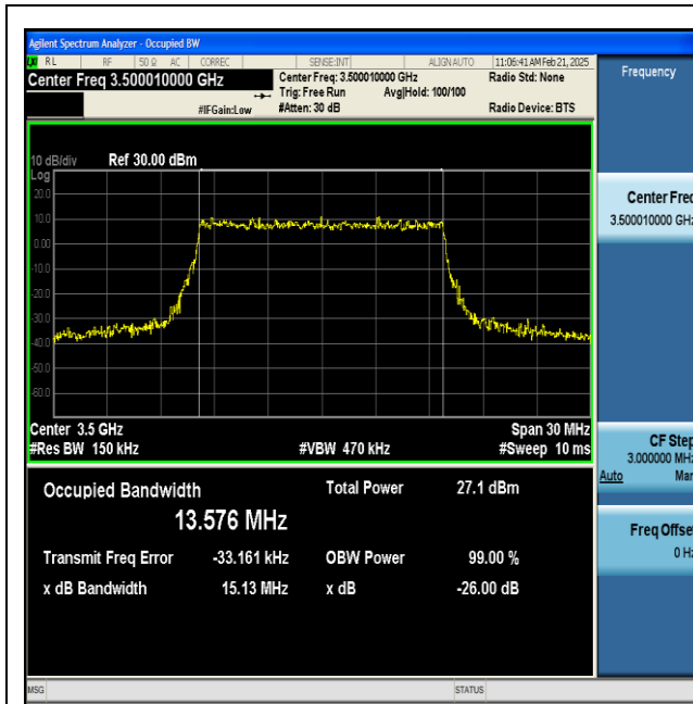
NTNV-n77(3450-3550)-PC2-30-15-M-CP-256QAM- Outer_Full-Ant1-PASS
