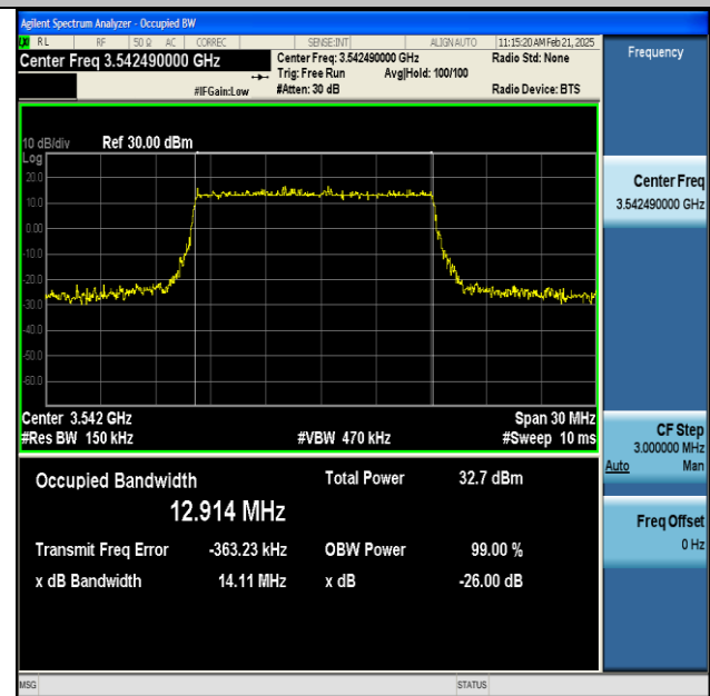
NTNV-n77(3450-3550)-PC2-30-15-H-DFT-16QAM- Outer_Full-Ant1-PASS
