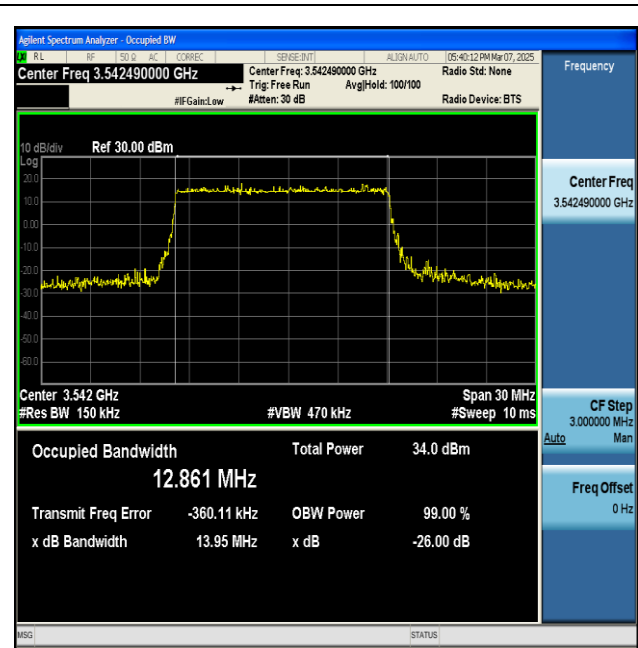
NTNV-n77(3450-3550)-PC2-30-15-H-DFT-BPSK- Outer_Full-Ant1-PASS
