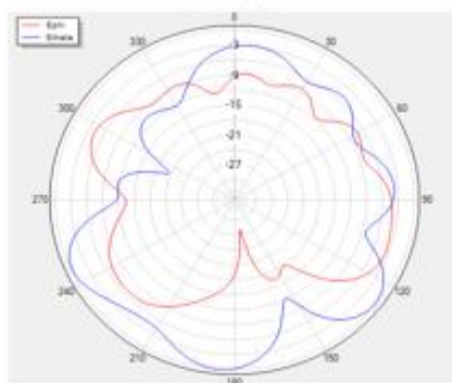
Theta=90 freq=2540MHz
