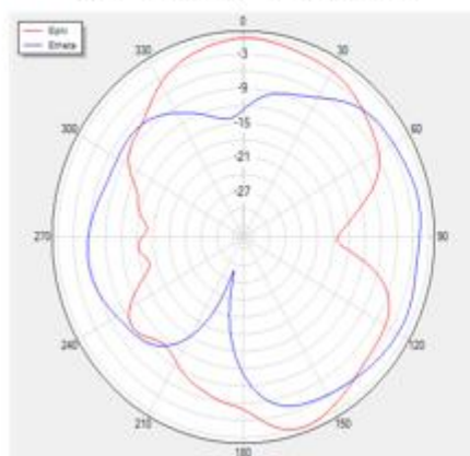
Phi=90 freq=1600MHz
