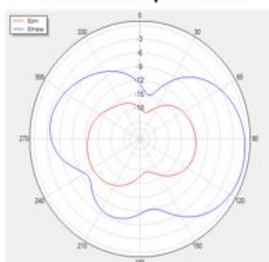
Theta=90 freq=800MHz
