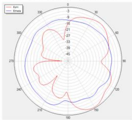
Phi=90 freq=2470MHz
