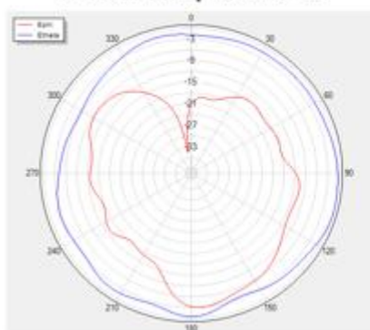
Phi=90 freq=800MHz
