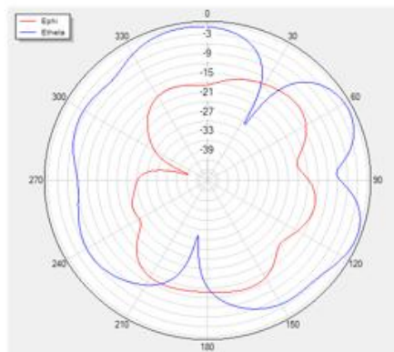
Theta=90 freq=2480MHz
