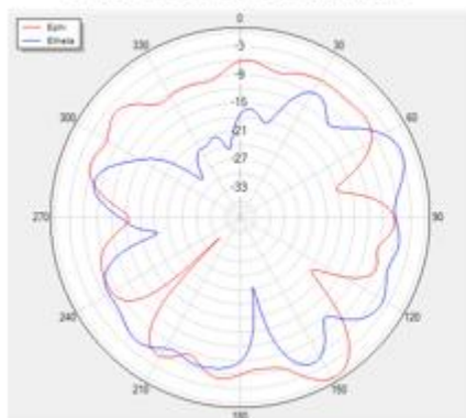
Phi=90 freq=2540MHz
