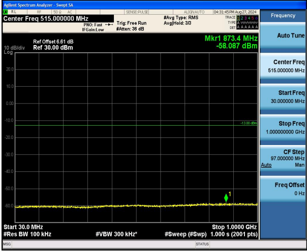
Band66_1.4MHz_QPSK_131979_1RB#0_30~1000_30~1000
