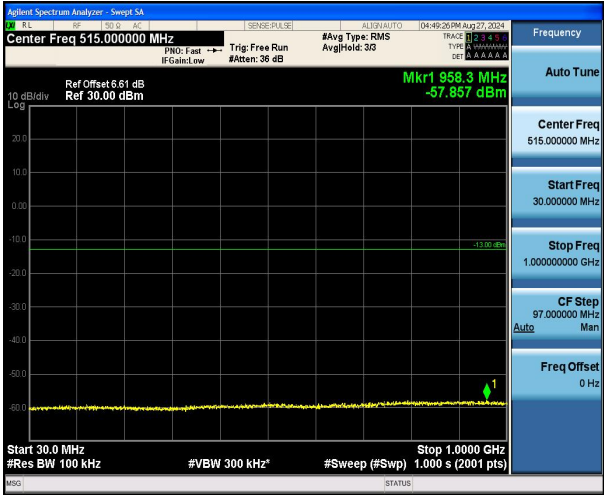
Band66_3MHz_16QAM_132322_1RB#0_30~1000_30~1000
