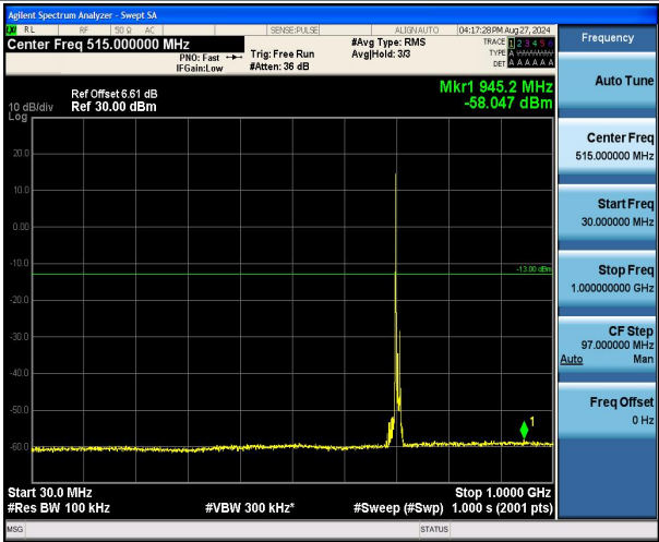
Band17_10MHz_16QAM_23800_1RB#0_30~1000_30~1000
