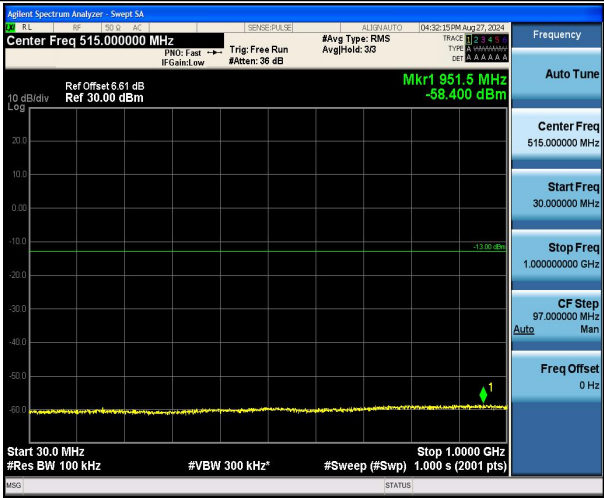
Band66_1.4MHz_16QAM_131979_1RB#0_30~1000_30~1000
