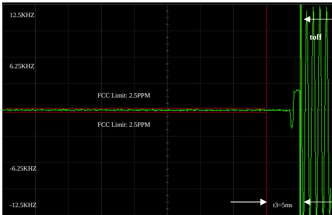
2 Watts, 173.975MHZ 12.5KHZ DE-KEY DECAY TIME
