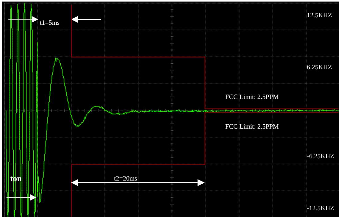
2 Watts, 148.025Mhz 12.5KHz KEY-UP ATTACK TIME
