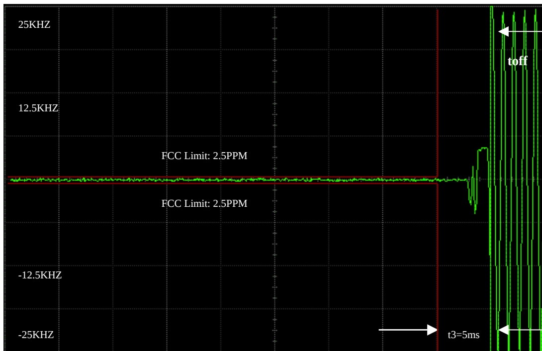
2 Watts, 173.975MHZ 25KHZ DE-KEY DECAY TIME
