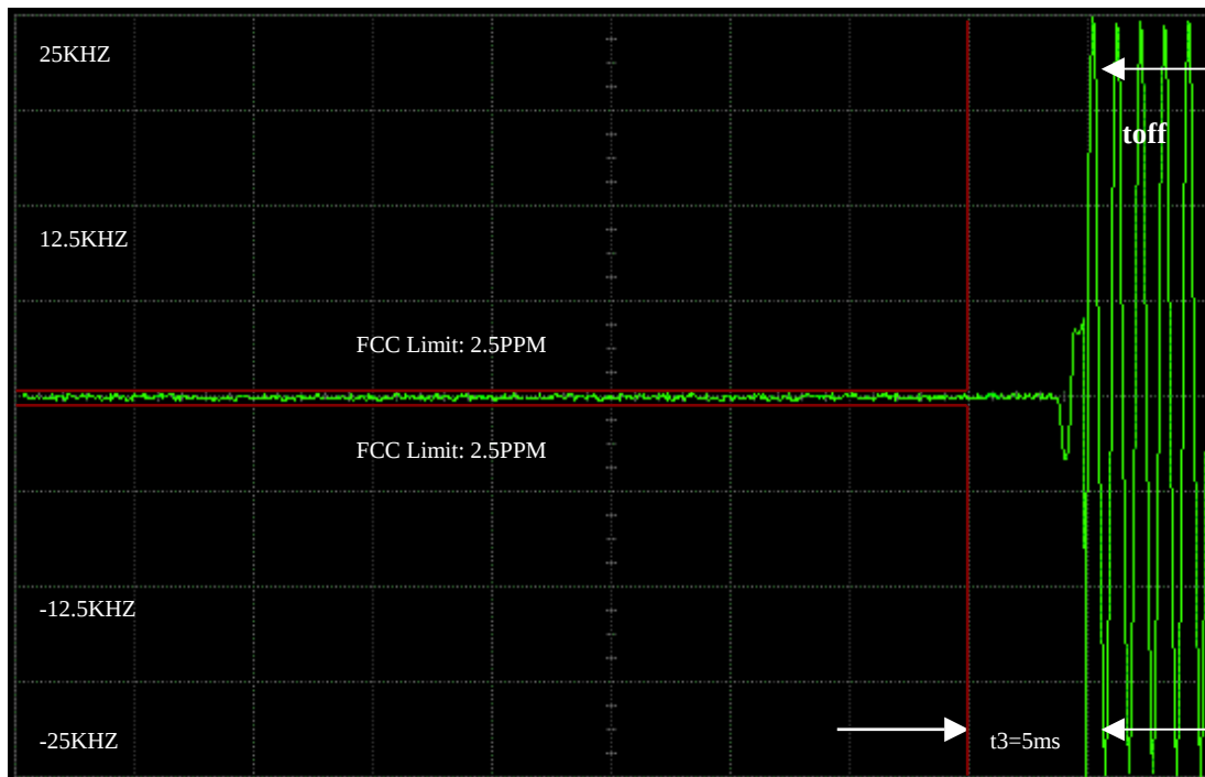
2 Watts, 162.025MHZ 25KHZ DE-KEY DECAY TIME
