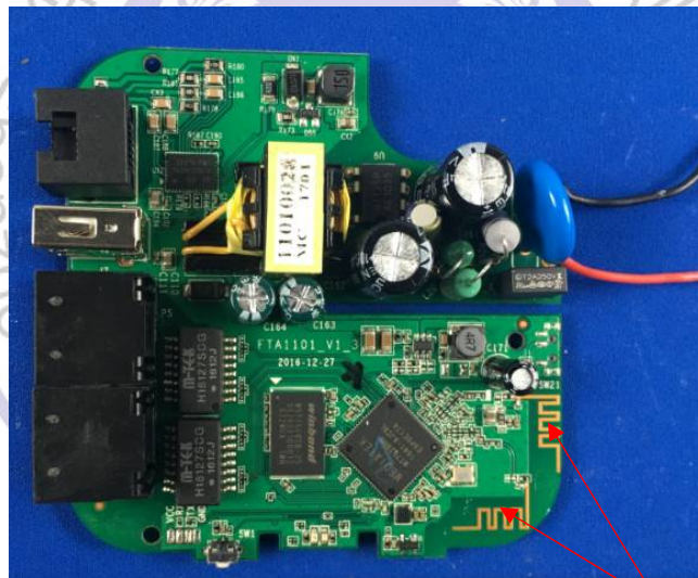
WIFI Antenna
