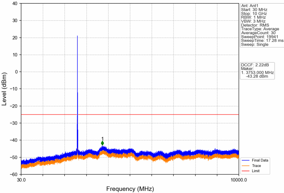
Band38_15MHz_16QAM_HCH_2612.5MHz_RB_1_0_NTNV
