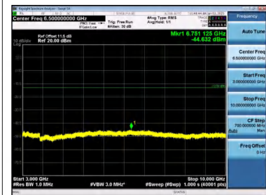
Band26(824-849)-3MHz-QPSK-26915-1RB#0-30 00~10000-PASS
