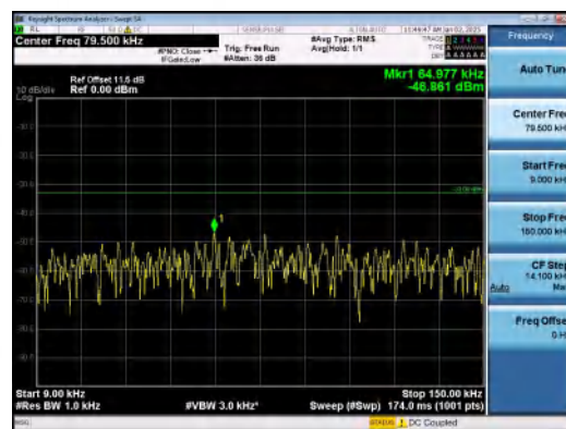
Band26(824-849)-3MHz-QPSK-26915-1RB#14-0 .009~0.15-PASS
