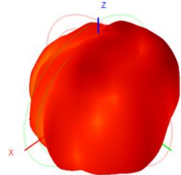
2450.0MHz H+V, Eff: 41.71%
