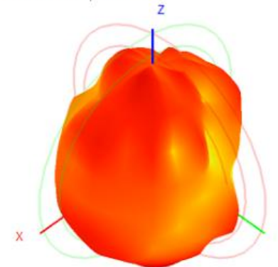
5850.0MHz H+V, Eff: 36.20%
