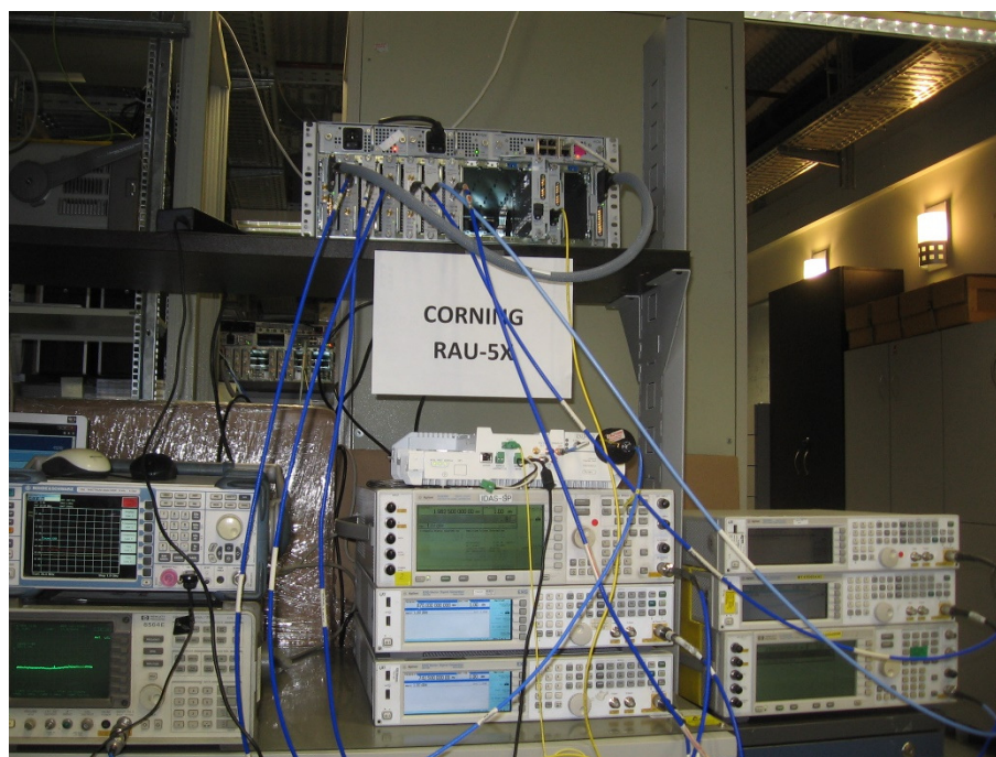
Intermodulated Conducted Emission Test
