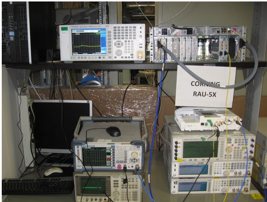
Conducted Emission From Antenna Port Test
