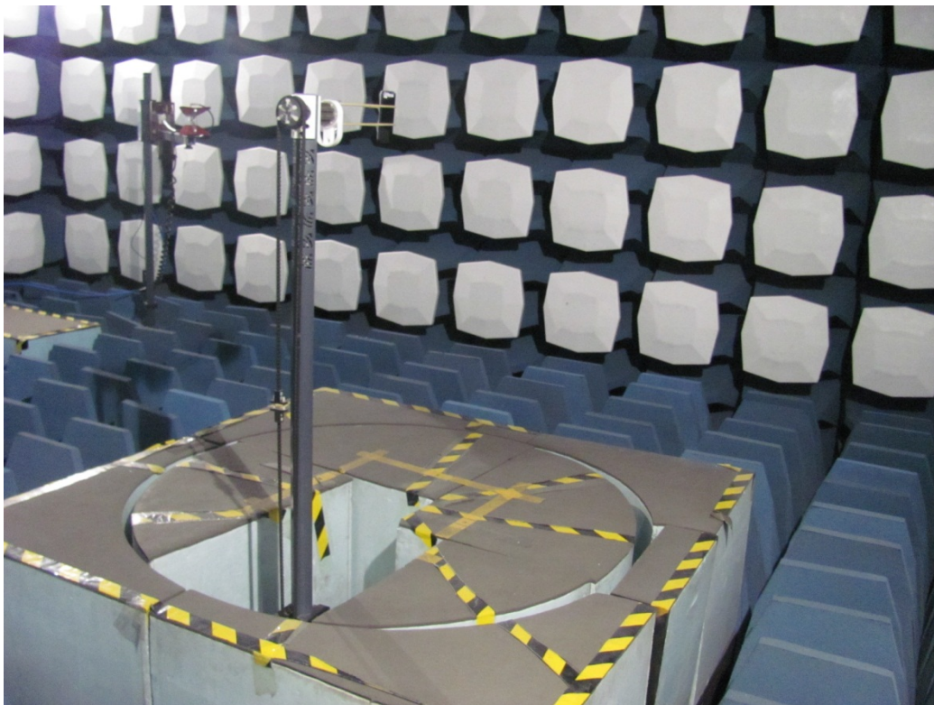
Pic F-3 Radiated Spurious Emission Test Layout
