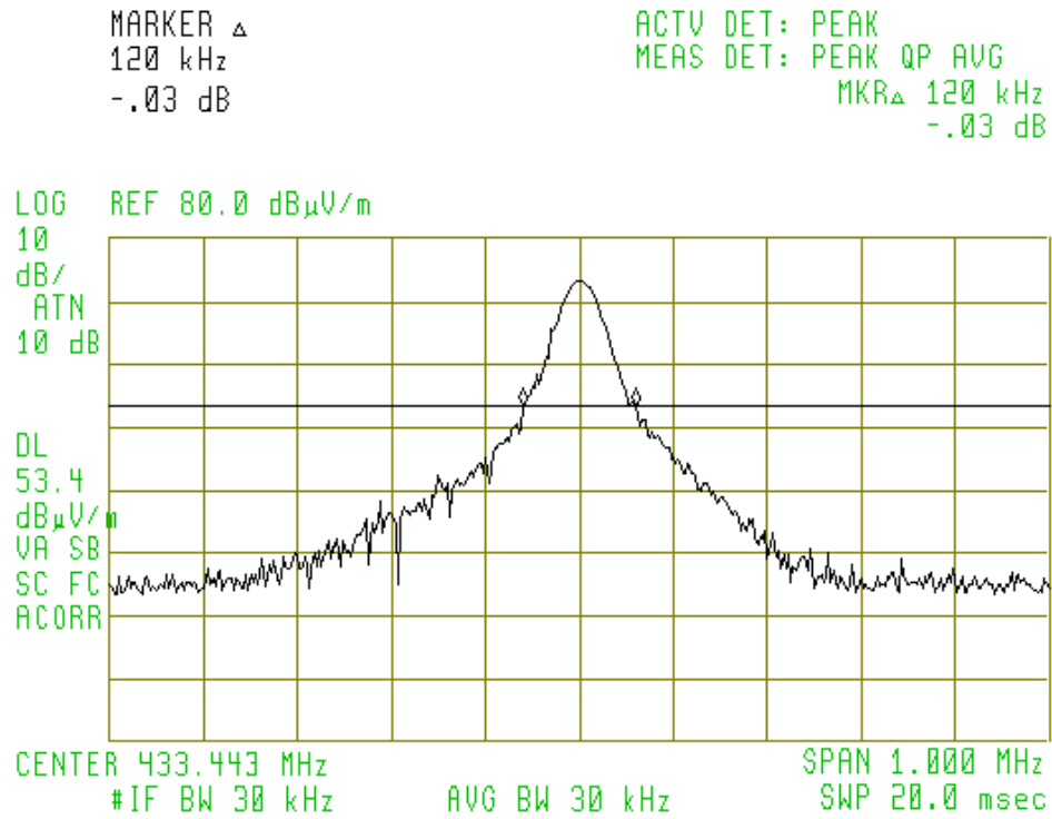
Figure 6.1 Occupied Bandwidth
