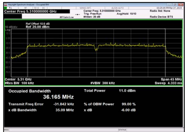
U-NII-2a 6dB Bandwidth-802.11ac(40MHz ,5310MHz,Ant1
