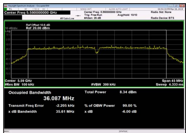
U-NII-2c 6dB Bandwidth-802.11n(40MHz) ,5590MHz,Ant1
