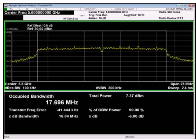
U-NII-2c 6dB Bandwidth-802.11n(20MHz) ,5600MHz,Ant1
