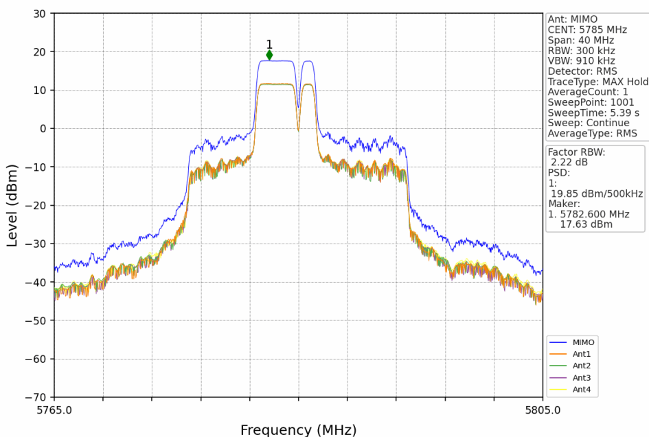
802.11be(EHT20)_MCH_5785MHz_RU52_Mid_MIMO_NTNV
