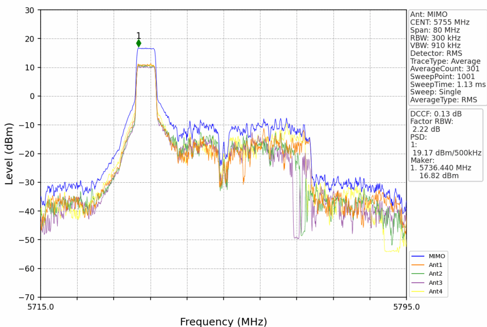
802.11ax(HEW40)_LCH_5755MHz_RU52_Left_MIMO_NTNV
