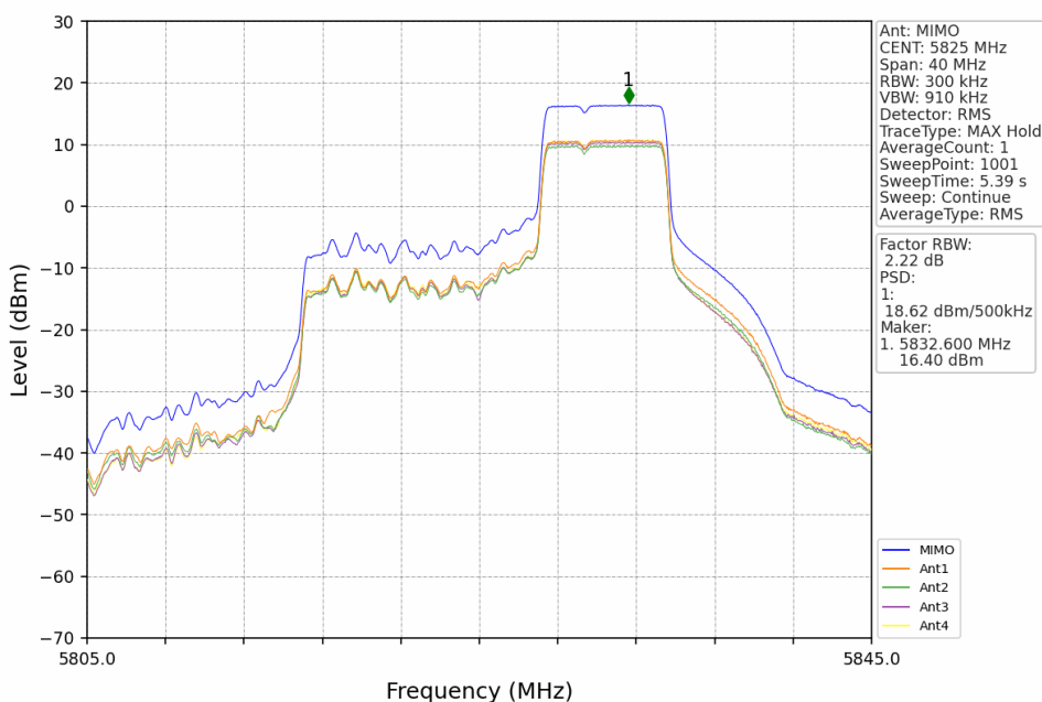
802.11ax(HEW20)_HCH_5825MHz_RU52+26_Right_MIMO_NTNV
