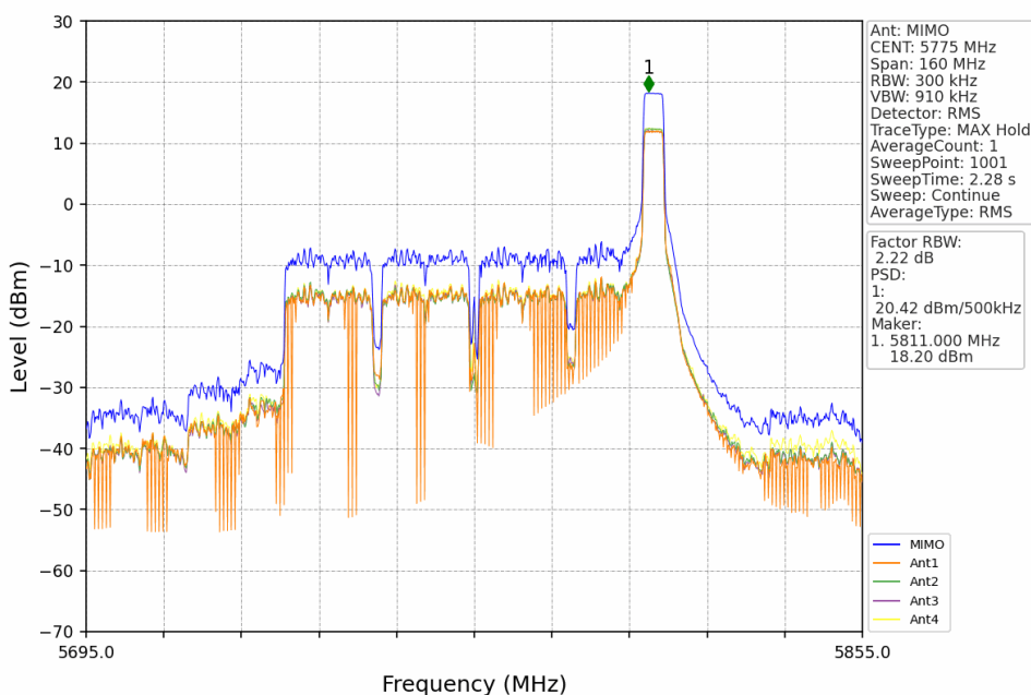
802.11ax(HEW80)_MCH_5775MHz_RU52_Right_MIMO_NTNV
