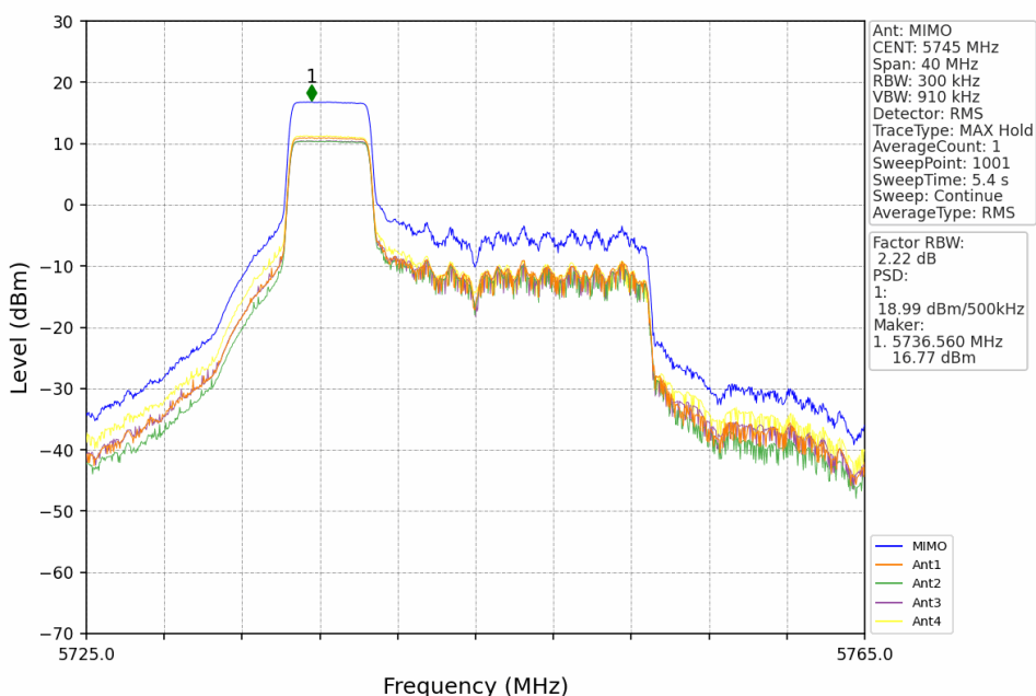
802.11ax(HEW20)_LCH_5745MHz_RU52+26_Left_MIMO_NTNV
