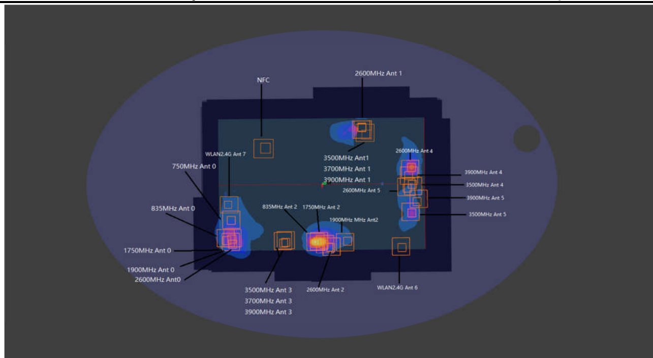
WWAN+WLAN2.4GHz Ant6+WLAN2.4GHz Ant7+NFC_Bottom Face 0mm
