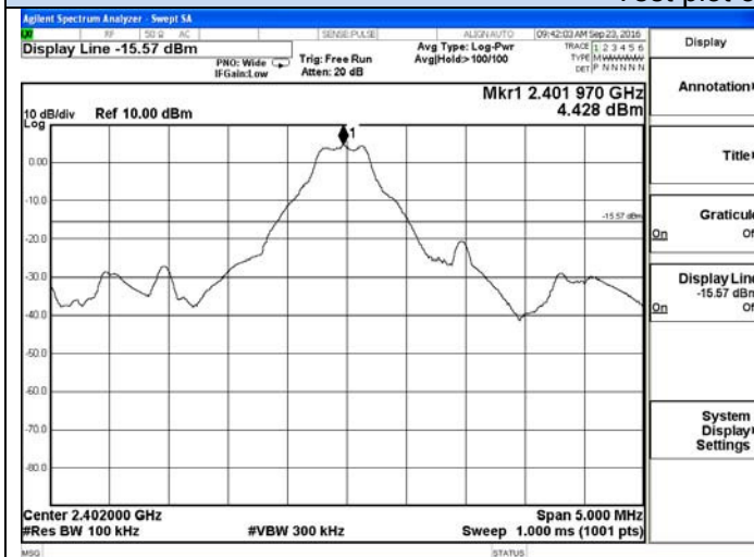
Reference of GFSK-Low channel
