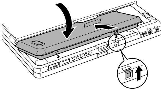
Figure 6-3 Installing the Battery Pack
