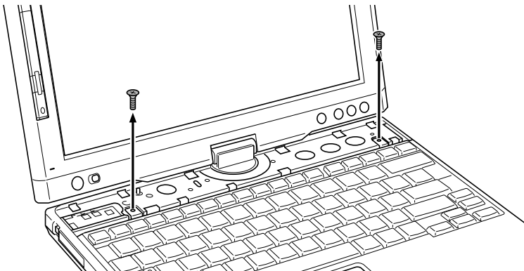
Figure 8-10 Removing the keyboard (1)
