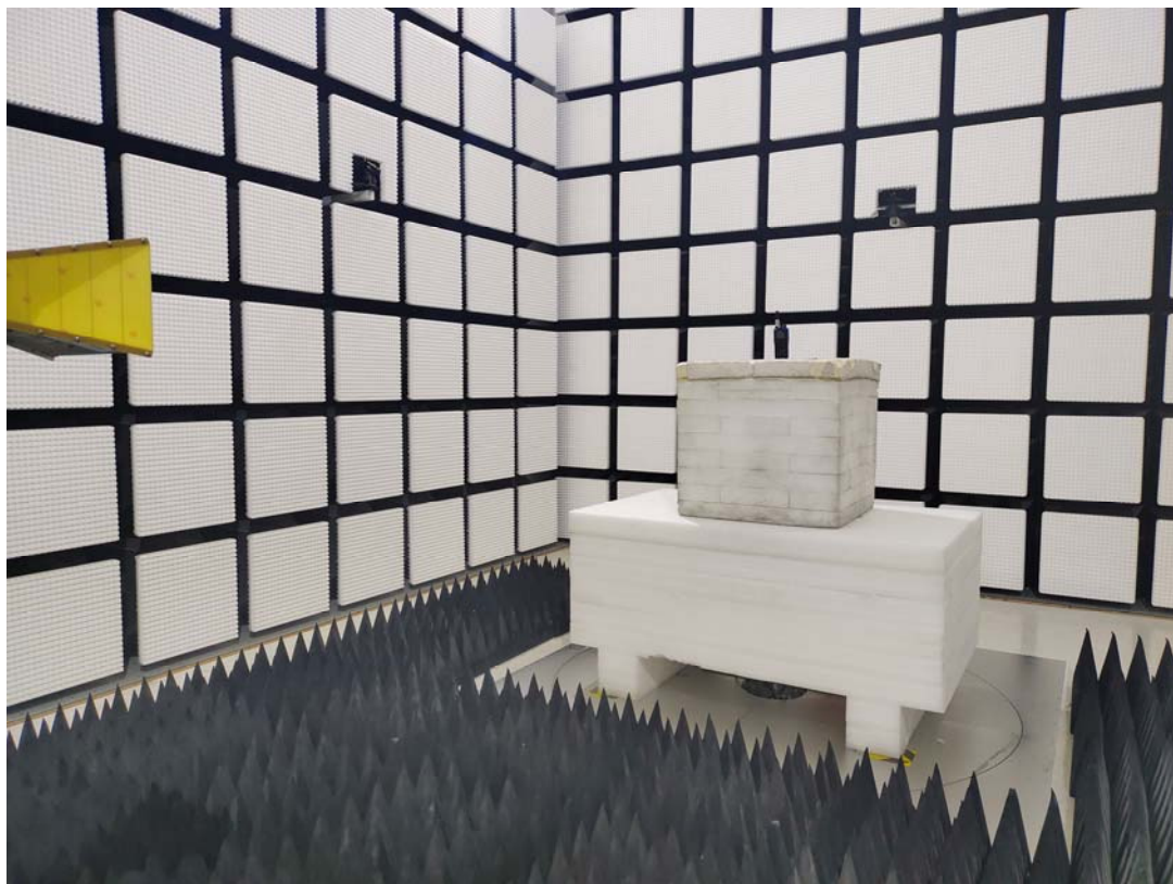
Radiated Emission Above 1GHz View- Model:DP810
