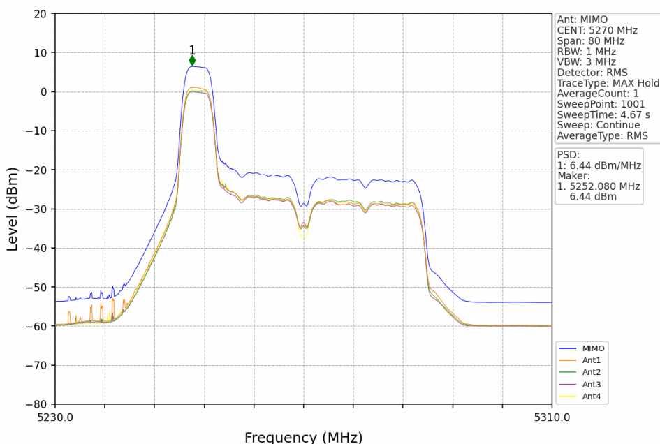
802.11ax(HEW40)_LCH_5270MHz_RU52+26_Left_MIMO_NTNV
