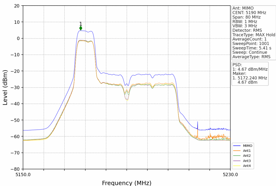
802.11ax(HEW40)_LCH_5190MHz_RU52+26_Left_MIMO_NTNV
