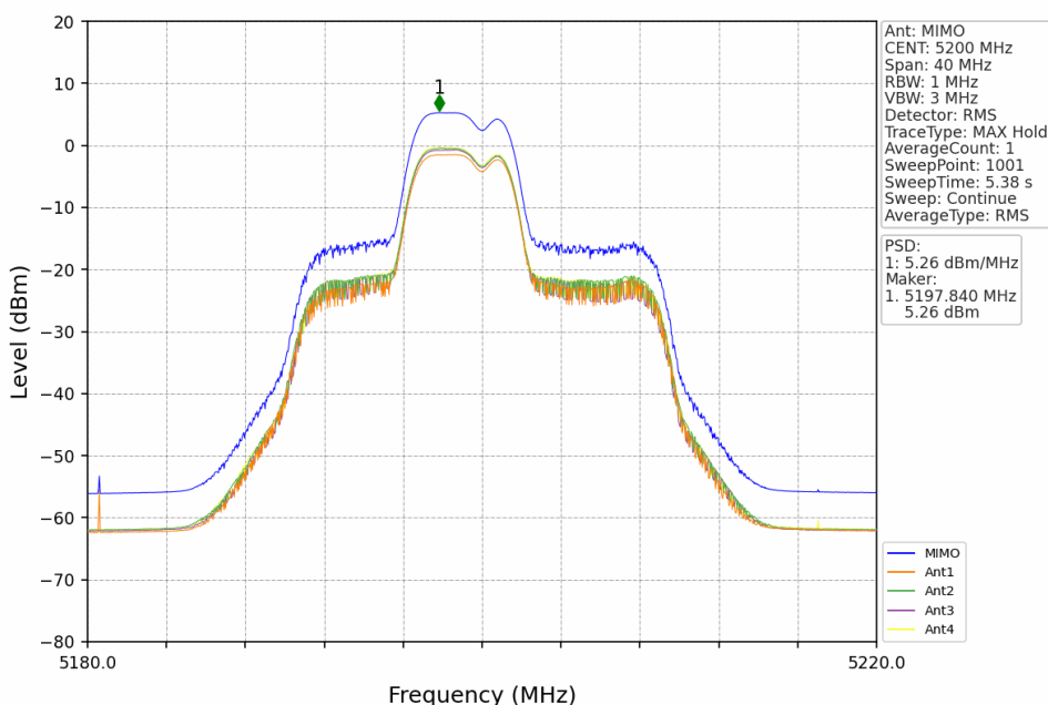
802.11ax(HEW20)_MCH_5200MHz_RU52+26_Mid_MIMO_NTNV
