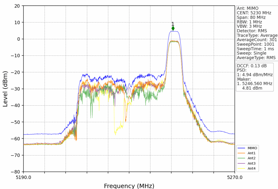
802.11ax(HEW40)_HCH_5230MHz_RU52_Right_MIMO_NTNV
