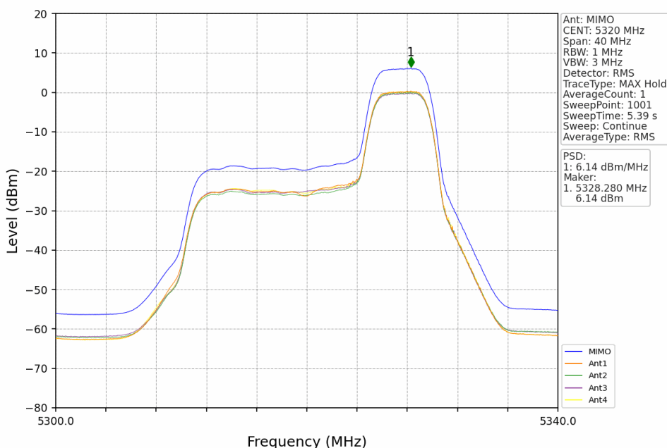
802.11ax(HEW20)_HCH_5320MHz_RU52+26_Right_MIMO_NTNV
