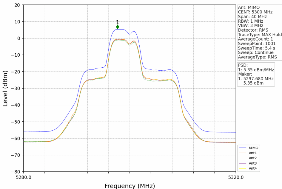
802.11ax(HEW20)_MCH_5300MHz_RU52_Mid_MIMO_NTNV
