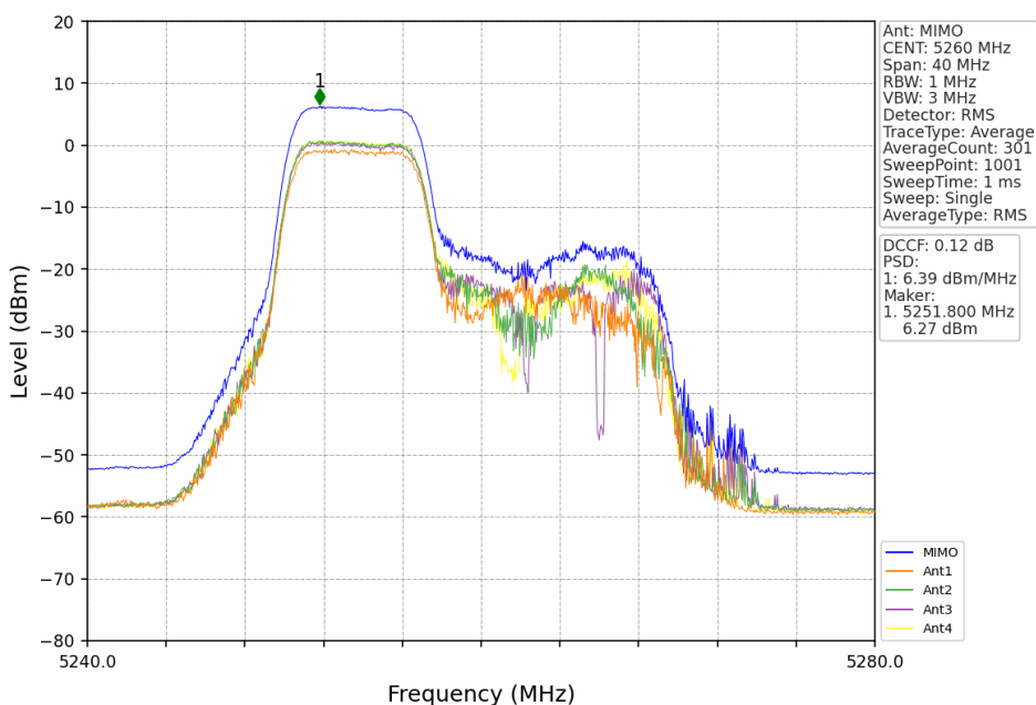
802.11ax(HEW20)_LCH_5260MHz_RU52+26_Left_MIMO_NTNV
