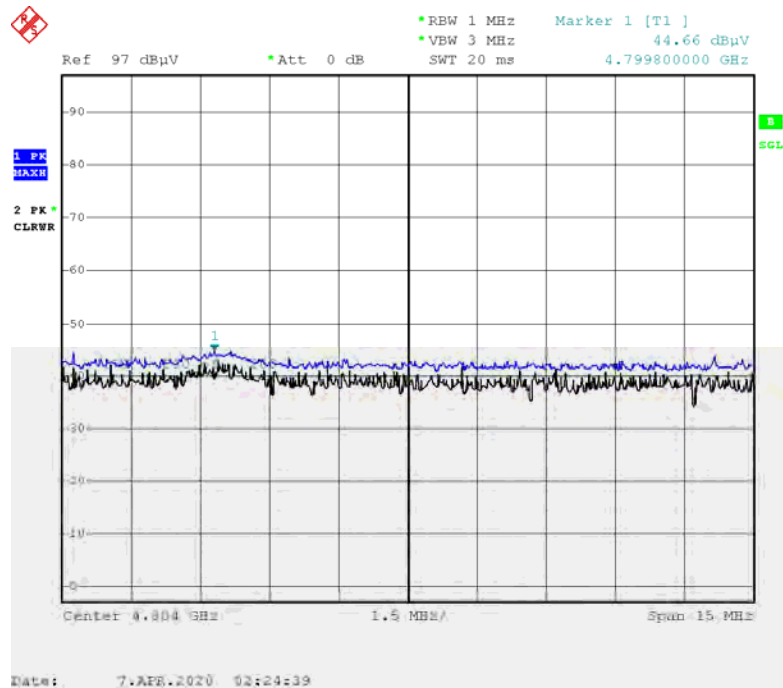
Radiated Spurious Emissions plot – Peak Reading ( \pi/4 DQPSK, Ch.0 2nd Harmonic, V)
