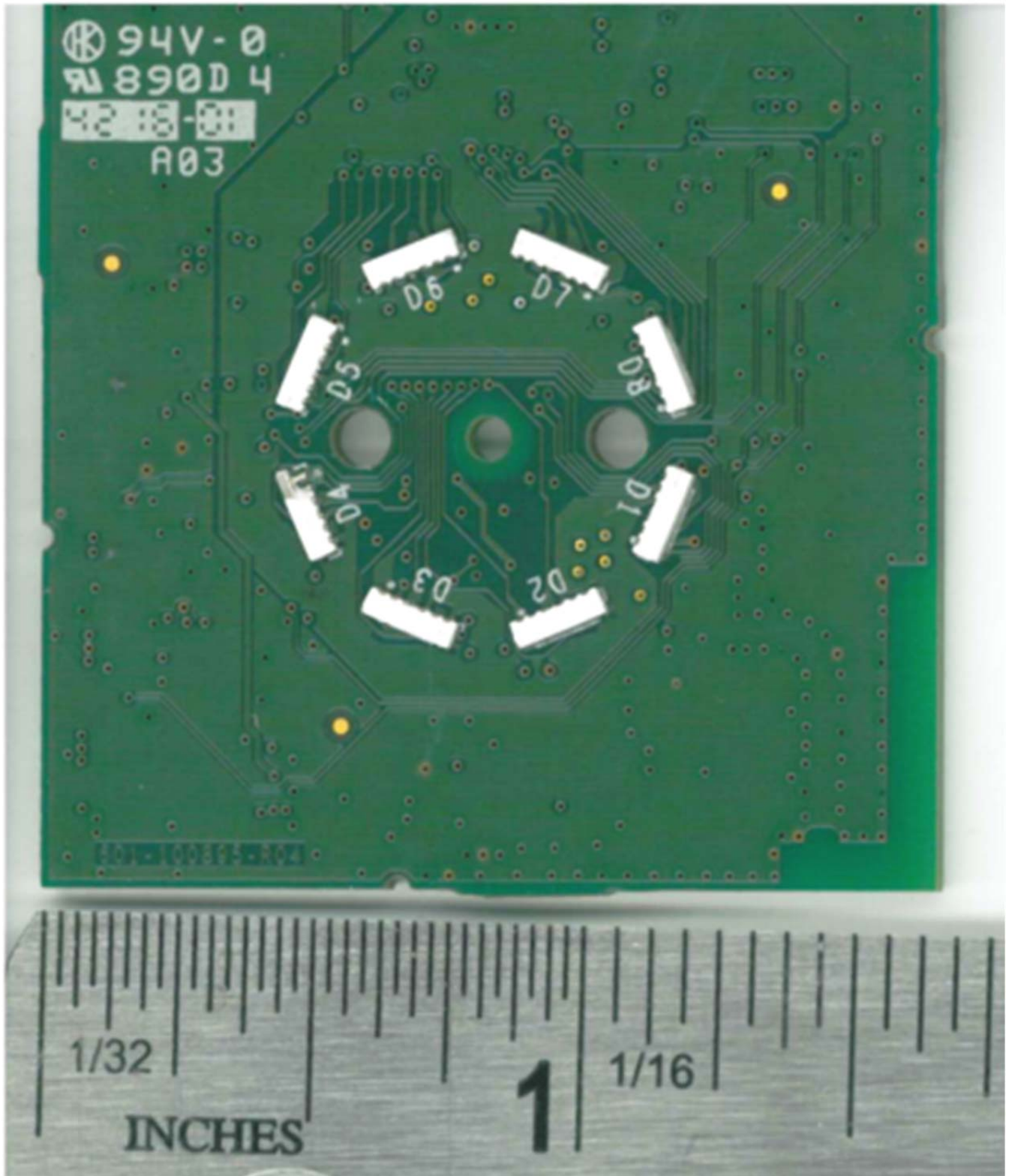
Main Board Top Side (LED Side) UBER Confidential
