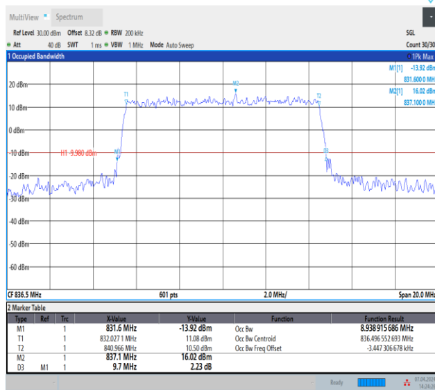
Band5-10MHz-QPSK-20525-50RB#0-PASS
