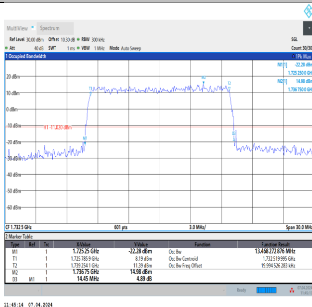
Band4-15MHz-16QAM-20175-75RB#0-PASS
