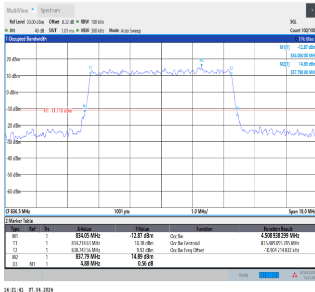
Band5-5MHz-16QAM-20525-25RB#0-PASS
