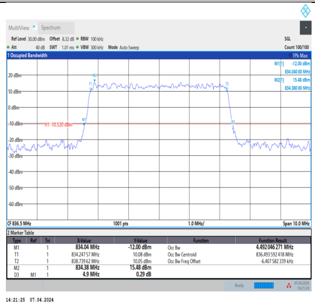
Band5-5MHz-QPSK-20525-25RB#0-PASS
