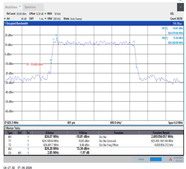
Band5-3MHz-QPSK-20415-15RB#0-PASS
