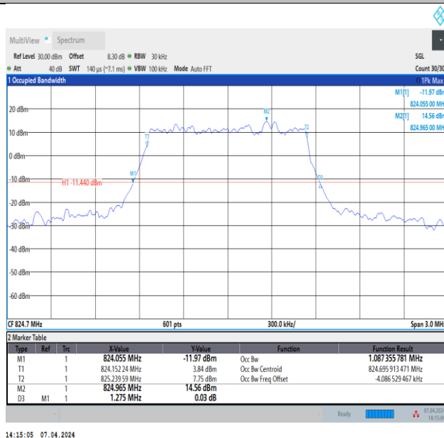
Band5-1.4MHz-64QAM-20407-6RB#0-PASS
