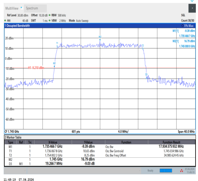
Band4-20MHz-64QAM-20300-100RB#0-PASS
