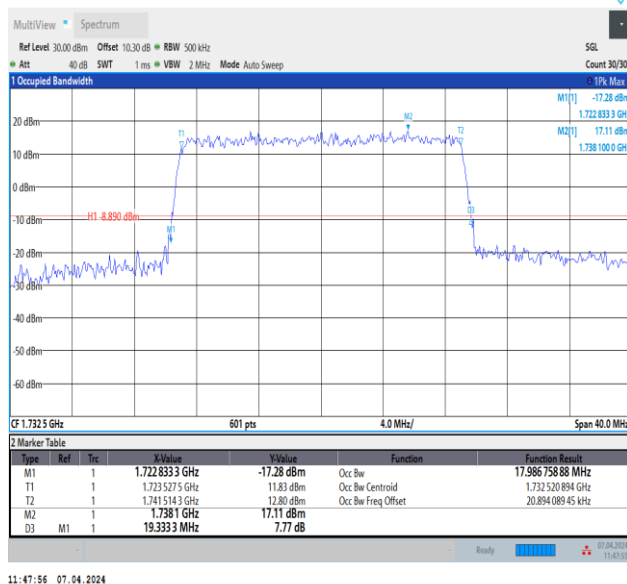
Band4-20MHz-QPSK-20175-100RB#0-PASS
