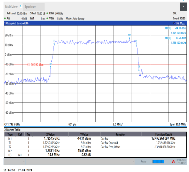
Band4-15MHz-QPSK-20175-75RB#0-PASS
