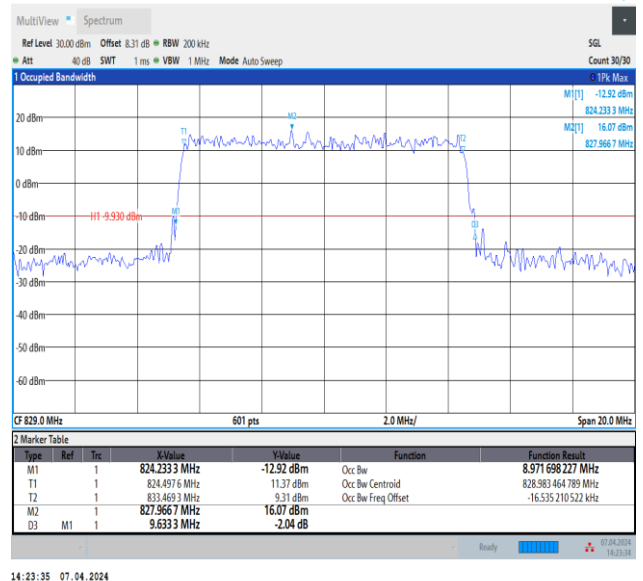
Band5-10MHz-QPSK-20450-50RB#0-PASS
