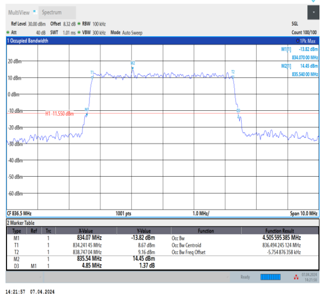
Band5-5MHz-64QAM-20525-25RB#0-PASS
