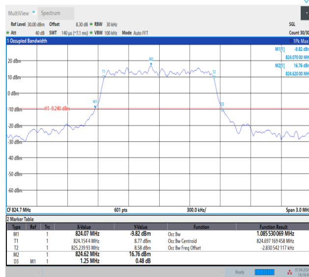
Band5-1.4MHz-16QAM-20407-6RB#0-PASS
