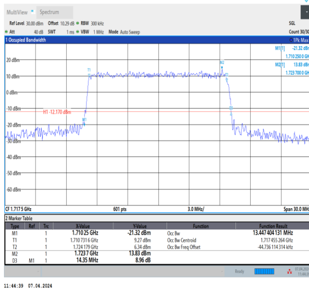
Band4-15MHz-64QAM-20025-75RB#0-PASS
