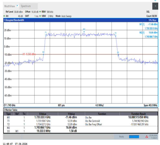
Band4-20MHz-QPSK-20300-100RB#0-PASS
