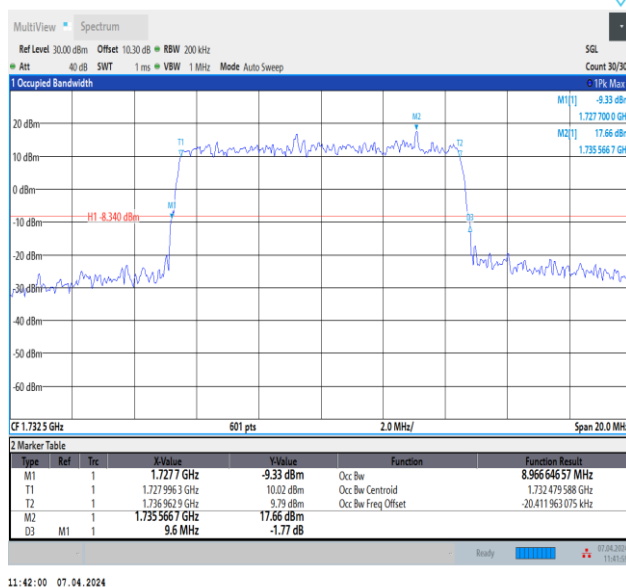
Band4-10MHz-QPSK-20175-50RB#0-PASS
