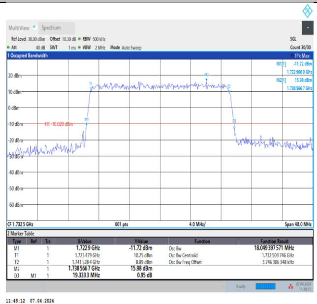
Band4-20MHz-16QAM-20175-100RB#0-PASS
