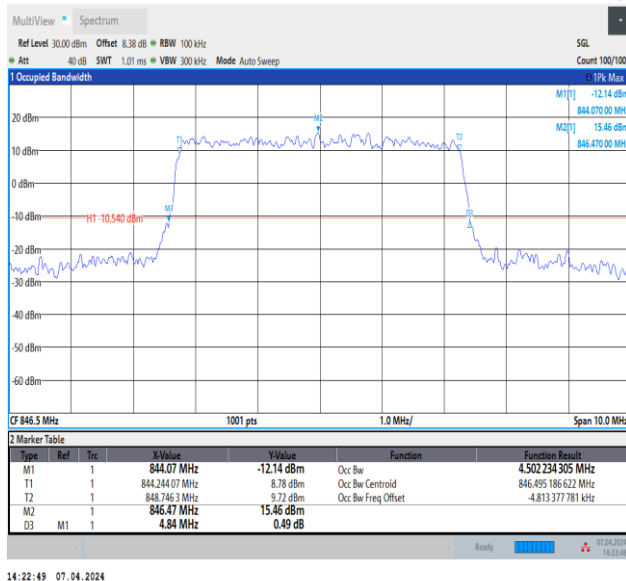
Band5-5MHz-64QAM-20625-25RB#0-PASS
