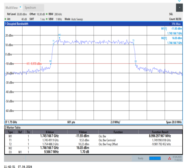
Band4-10MHz-QPSK-20350-50RB#0-PASS
