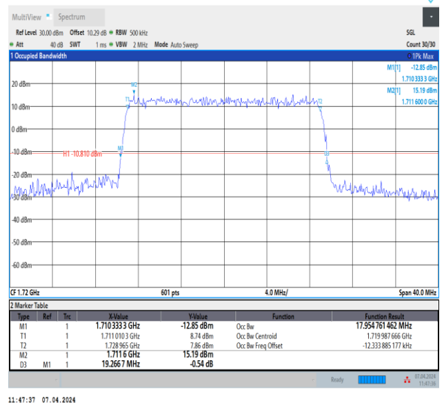
Band4-20MHz-64QAM-20050-100RB#0-PASS
