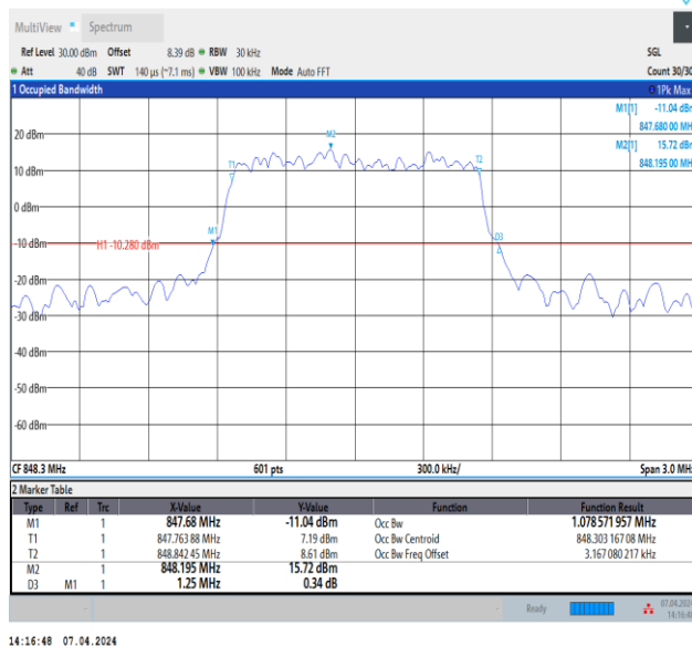
Band5-1.4MHz-64QAM-20643-6RB#0-PASS
