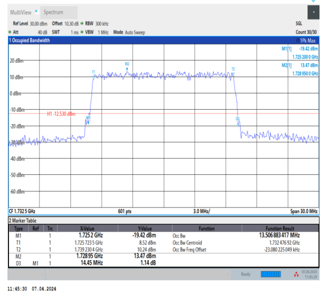
Band4-15MHz-64QAM-20175-75RB#0-PASS
