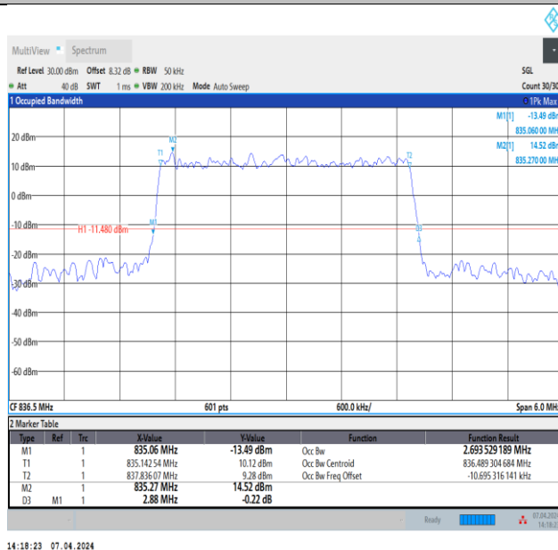
Band5-3MHz-QPSK-20525-15RB#0-PASS
