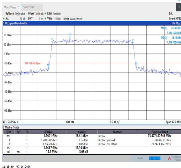
Band4-15MHz-QPSK-20325-75RB#0-PASS
