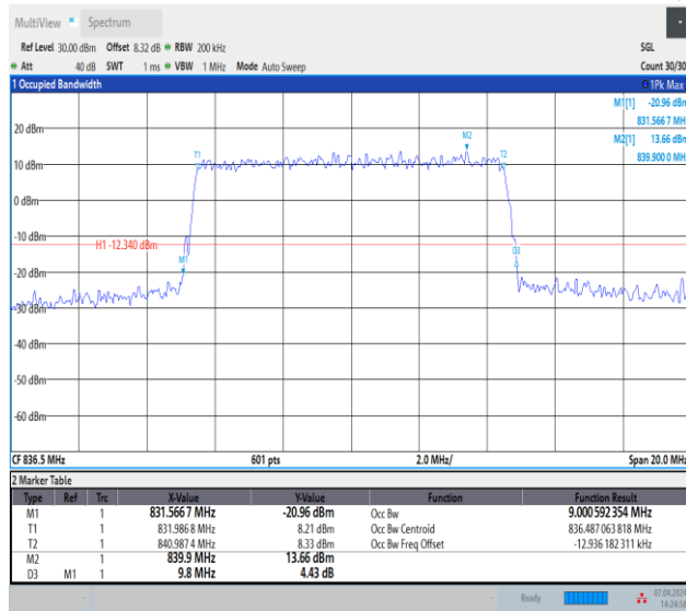
Band5-10MHz-64QAM-20525-50RB#0-PASS
