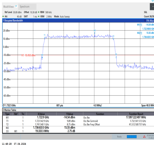
Band4-20MHz-64QAM-20175-100RB#0-PASS
