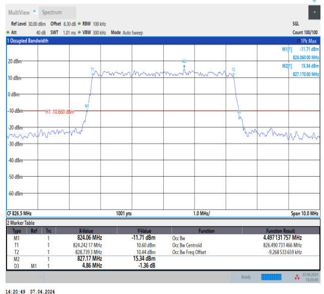
Band5-5MHz-16QAM-20425-25RB#0-PASS
