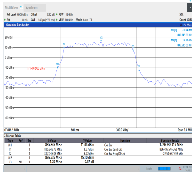
Band5-1.4MHz-QPSK-20525-6RB#0-PASS
