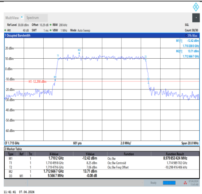
Band4-10MHz-64QAM-20000-50RB#0-PASS
