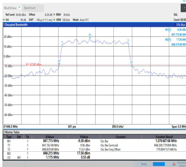
Band5-1.4MHz-QPSK-20643-6RB#0-PASS
