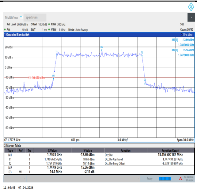
Band4-15MHz-16QAM-20325-75RB#0-PASS
