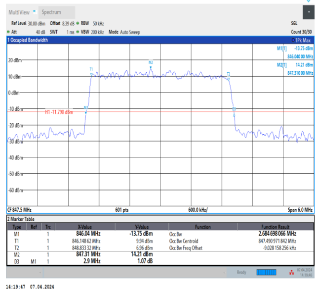
Band5-3MHz-64QAM-20635-15RB#0-PASS
