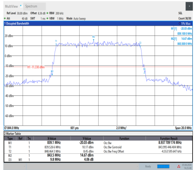
Band5-10MHz-64QAM-20600-50RB#0-PASS
