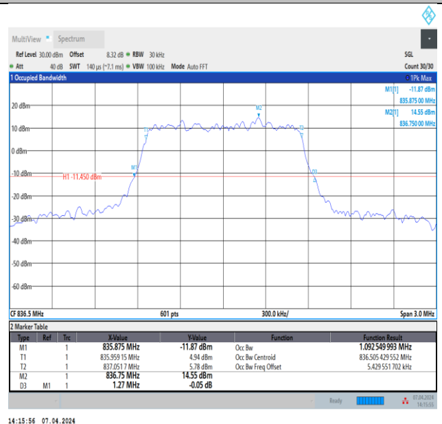
Band5-1.4MHz-64QAM-20525-6RB#0-PASS
