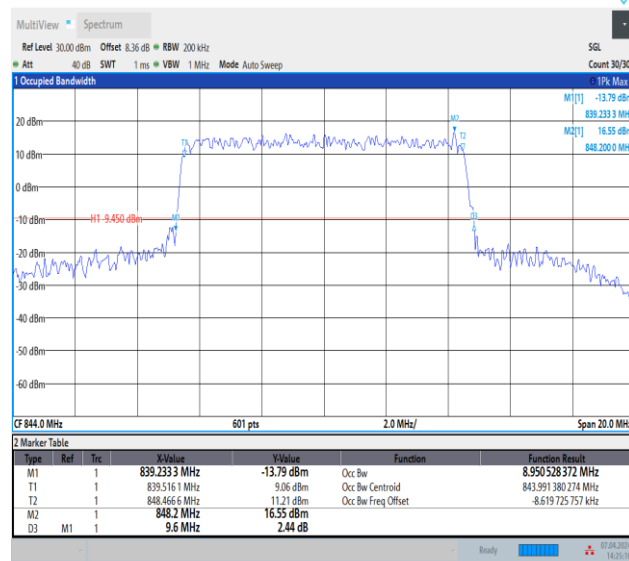
Band5-10MHz-QPSK-20600-50RB#0-PASS
