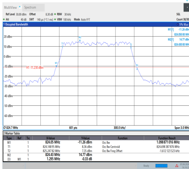
Band5-1.4MHz-QPSK-20407-6RB#0-PASS
