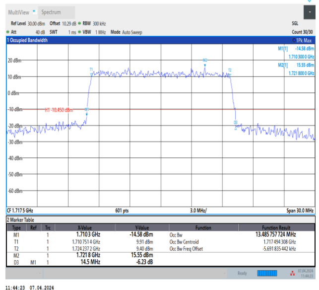
Band4-15MHz-16QAM-20025-75RB#0-PASS
