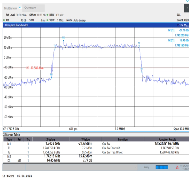
Band4-15MHz-64QAM-20325-75RB#0-PASS
