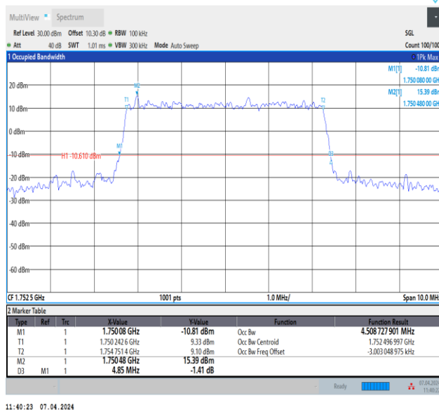
Band4-5MHz-64QAM-20375-25RB#0-PASS
