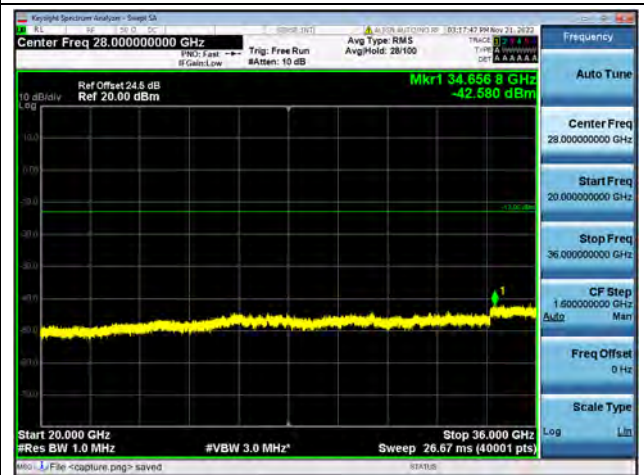
Band42-20G-36G / 10MHz / Low CH / 64QAM
