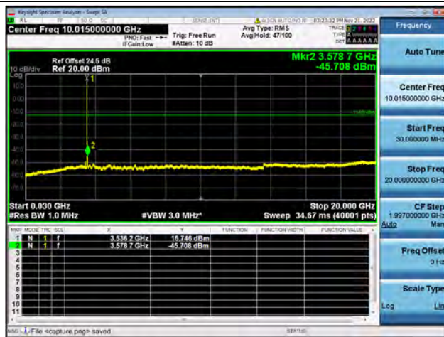
Band42-30M-20G / 15MHz / High CH / 16QAM
