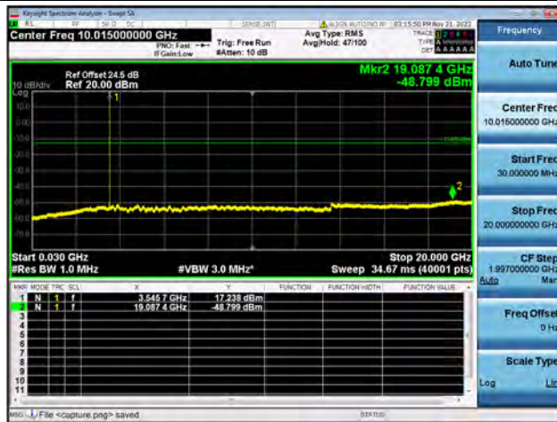
Band42-30M-20G / 5MHz / High CH / 16QAM
