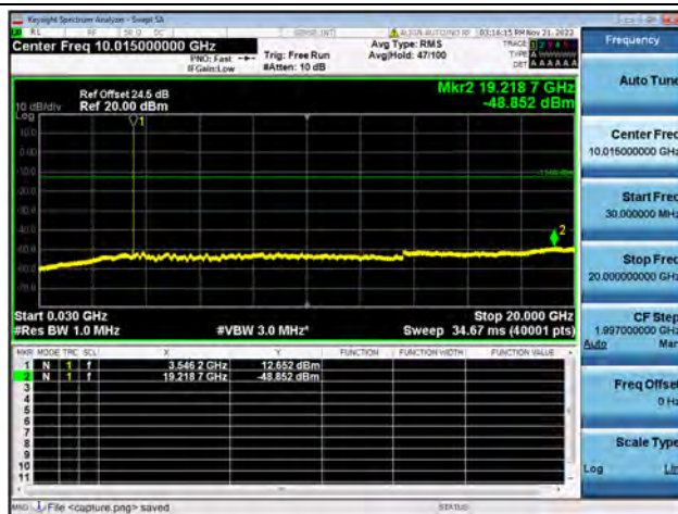
Band42-30M-20G / 5MHz / High CH / 64QAM
