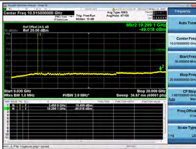
Band42-30M-20G / 5MHz / Low CH / 16QAM
