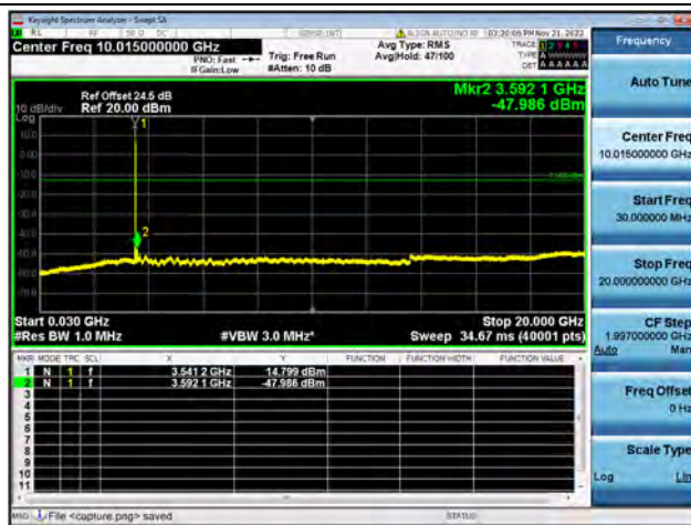
Band42-30M-20G / 10MHz / High CH / 64QAM
