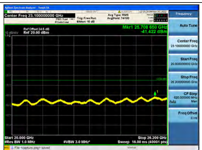
Band38-20G-26G / 5MHz / Low CH / QPSK
