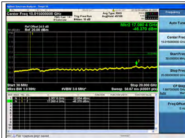
Band30-30M-20G / 5MHz / Mid CH / QPSK
