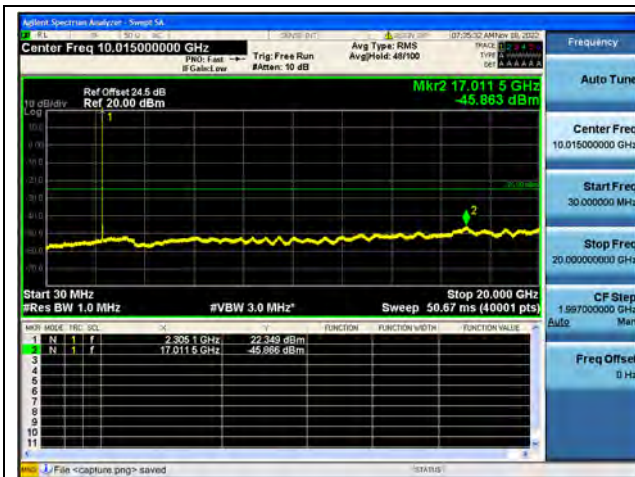
Band30-30M-20G / 10MHz / Low CH / QPSK
