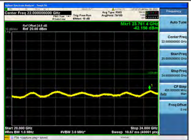
Band30-20G-24G / 10MHz / Mid CH / 16QAM
