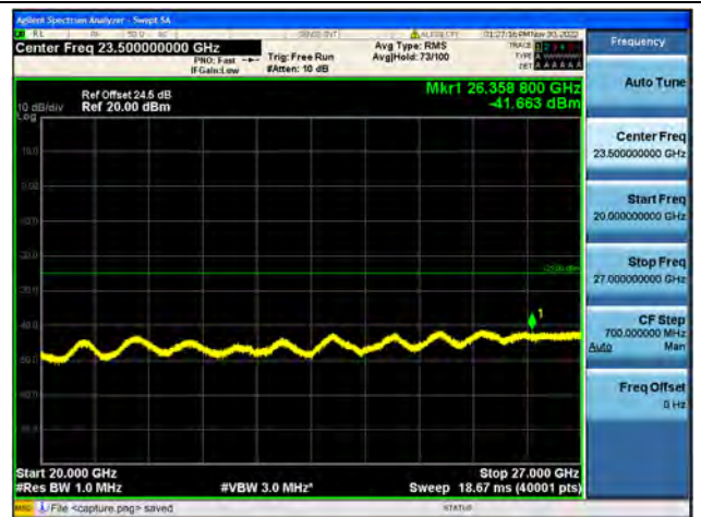
Band41-20G-27G / 20MHz / High CH / 16QAM
