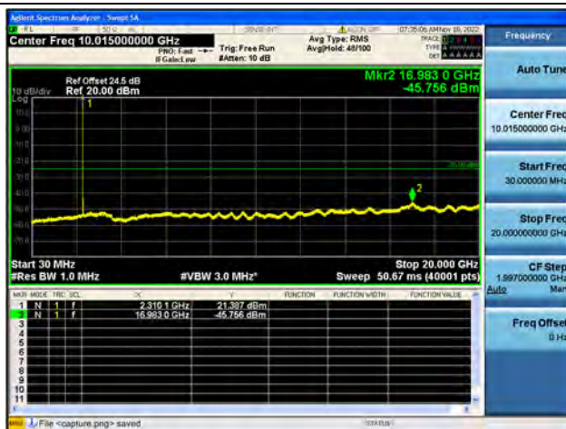
Band30-30M-20G / 5MHz / High CH / 64QAM
