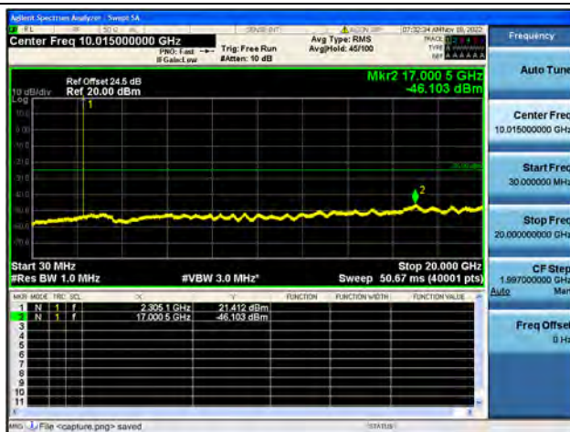
Band30-30M-20G / 5MHz / Low CH / 64QAM
