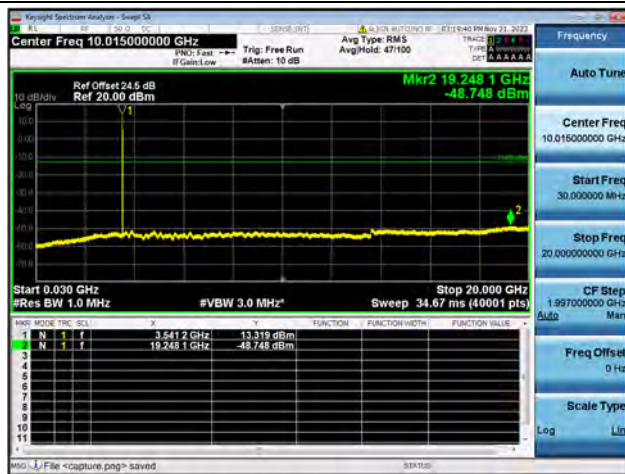
Band42-30M-20G / 10MHz / High CH / 16QAM
