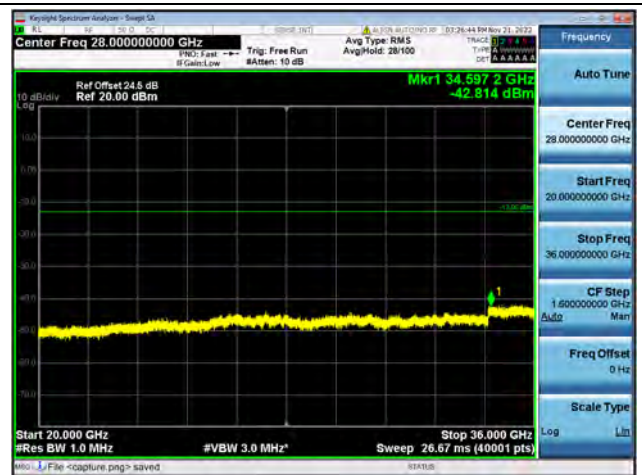
Band42-20G-36G / 20MHz / Mid CH / 64QAM
