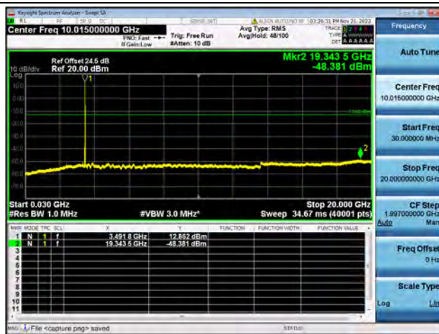
Band42-30M-20G / 20MHz / Mid CH / 64QAM
