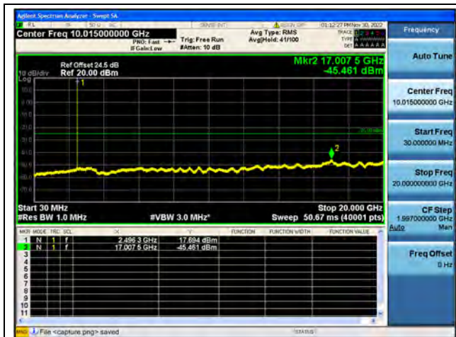
Band41-30M-20G / 5MHz / Low CH / QPSK
