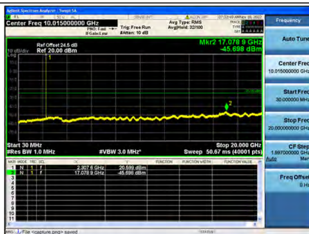
Band30-30M-20G / 5MHz / Mid CH / 64QAM
