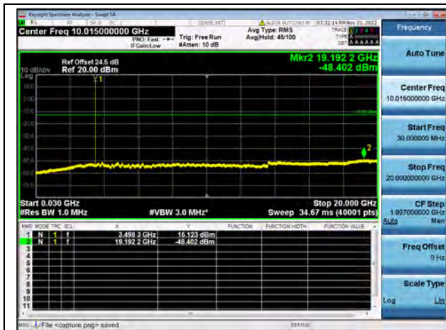
Band42-30M-20G / 5MHz / Mid CH / QPSK
