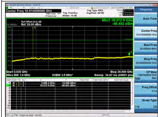
Band42-30M-20G / 5MHz / Mid CH / 16QAM
