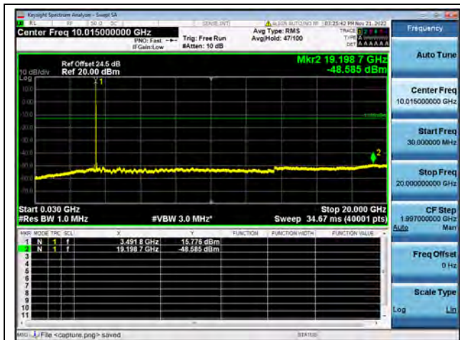
Band42-30M-20G / 20MHz / Mid CH / QPSK
