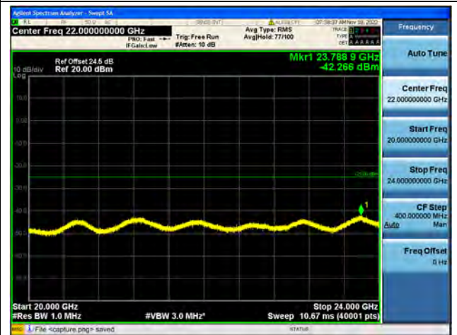
Band30-20G-24G / 10MHz / High CH / 16QAM
