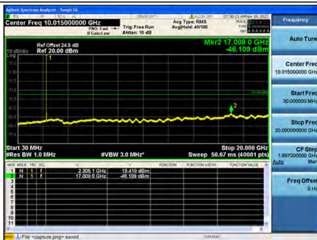
Band30-30M-20G / 10MHz / Low CH / 64QAM
