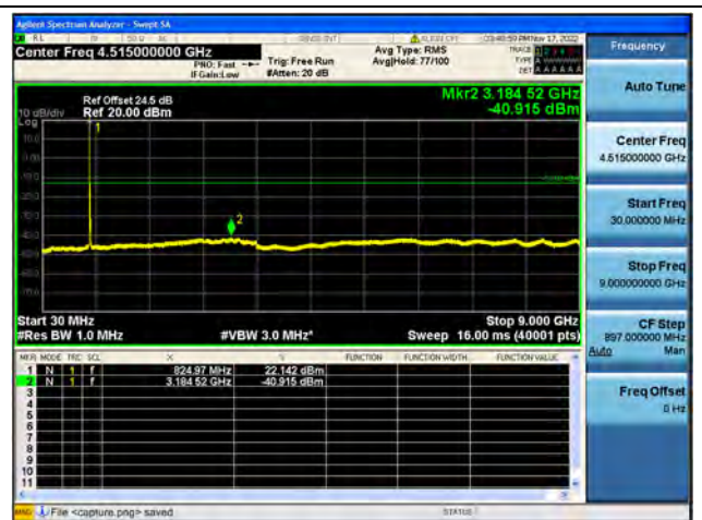
Band26Part22 / 15MHz / Low CH / 16QAM
