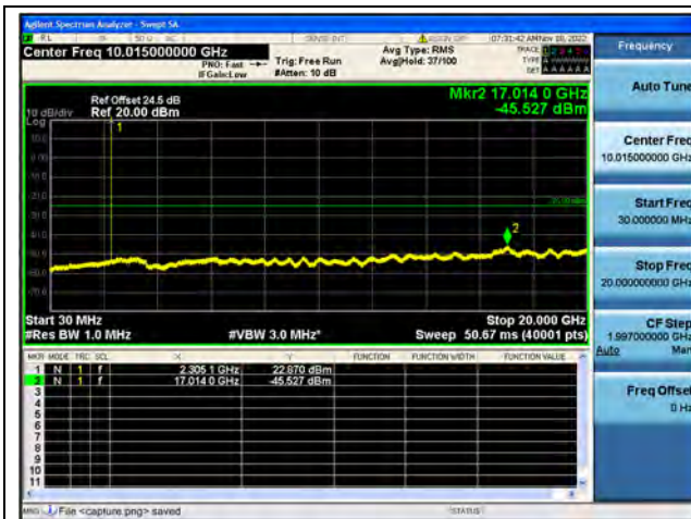
Band30-30M-20G / 5MHz / Low CH / QPSK
