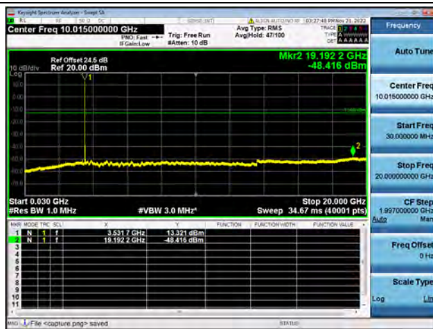
Band42-30M-20G / 20MHz / High CH / 64QAM
