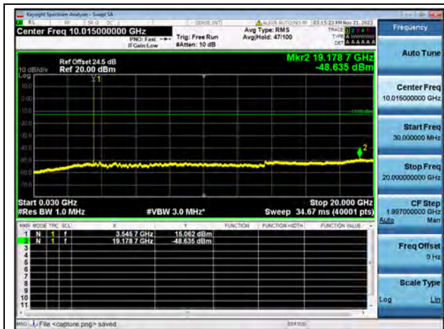
Band42-30M-20G / 5MHz / High CH / QPSK
