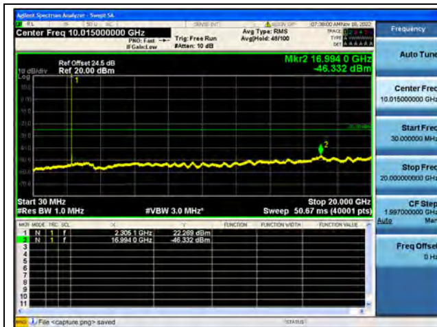
Band30-30M-20G / 10MHz / High CH / QPSK
