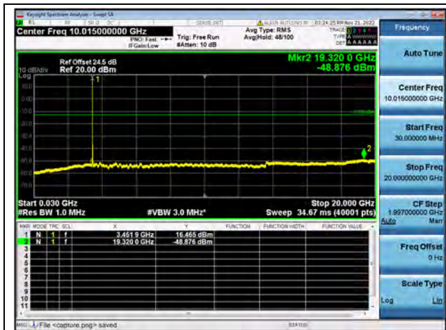
Band42-30M-20G / 20MHz / Low CH / QPSK
