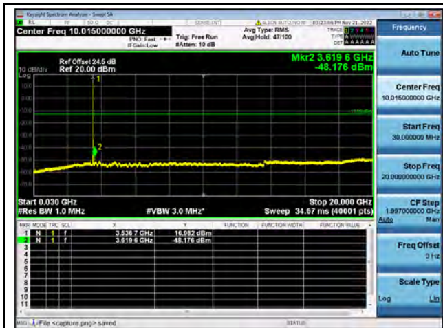
Band42-30M-20G / 15MHz / High CH / QPSK
