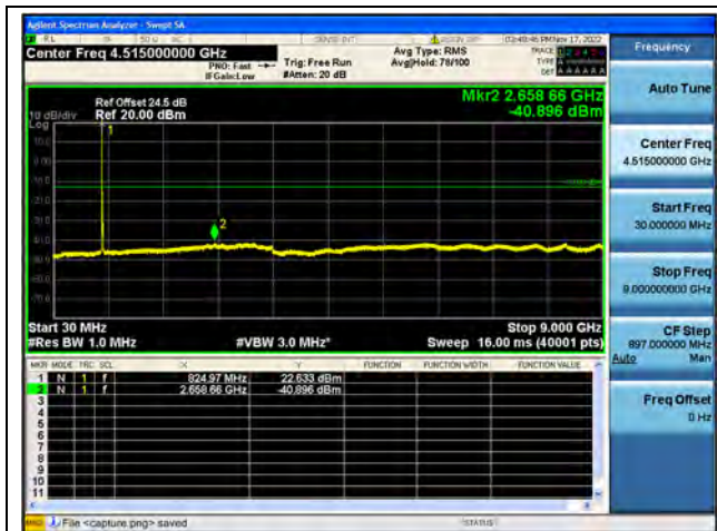
Band26Part22 / 15MHz / Low CH / QPSK
