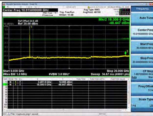
Band42-30M-20G / 20MHz / Mid CH / 16QAM
