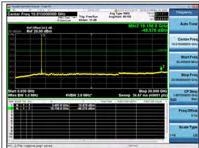
Band42-30M-20G / 15MHz / Mid CH / QPSK
