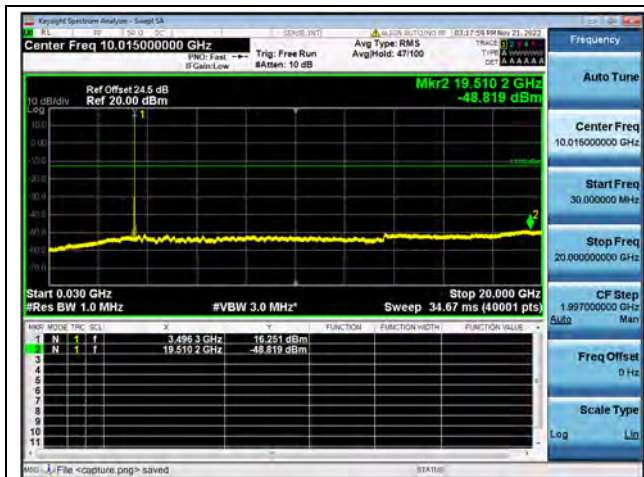
Band42-30M-20G / 10MHz / Mid CH / QPSK
