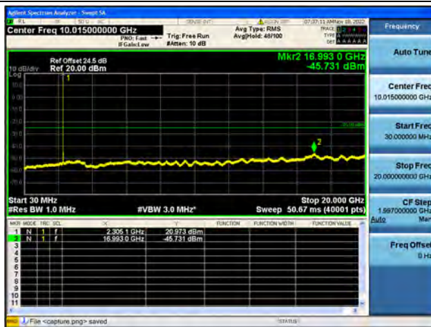
Band30-30M-20G / 10MHz / Mid CH / 16QAM
