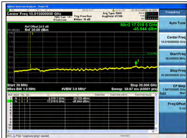
Band30-30M-20G / 5MHz / High CH / QPSK
