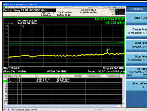
Band30-30M-20G / 5MHz / Mid CH / 16QAM
