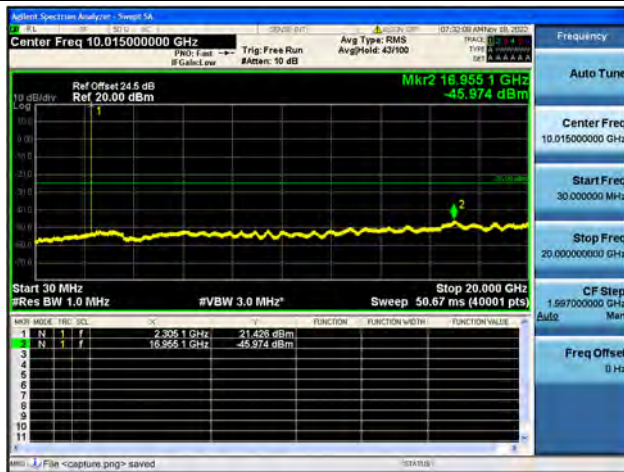
Band30-30M-20G / 5MHz / Low CH / 16QAM
