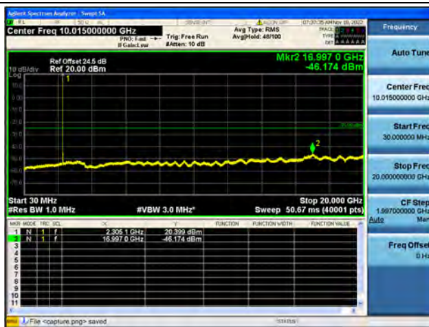
Band30-30M-20G / 10MHz / Mid CH / 64QAM
