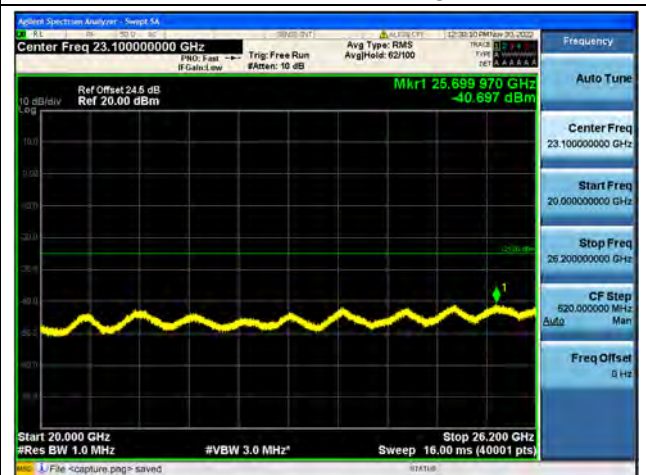
Band38-20G-26G / 20MHz / High CH / 16QAM
