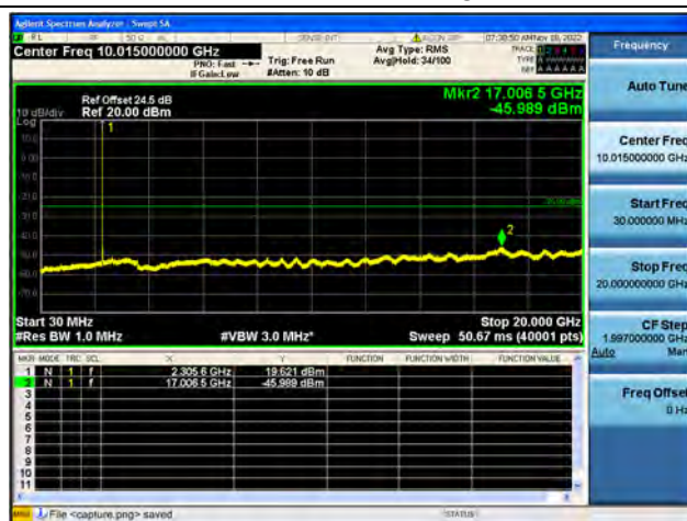
Band30-30M-20G / 10MHz / High CH / 64QAM
