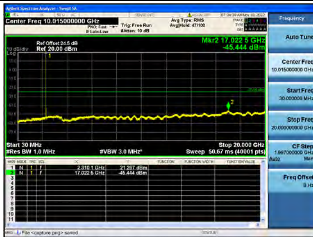
Band30-30M-20G / 5MHz / High CH / 16QAM
