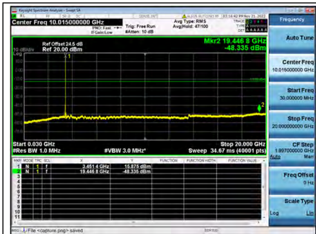
Band42-30M-20G / 10MHz / Low CH / QPSK
