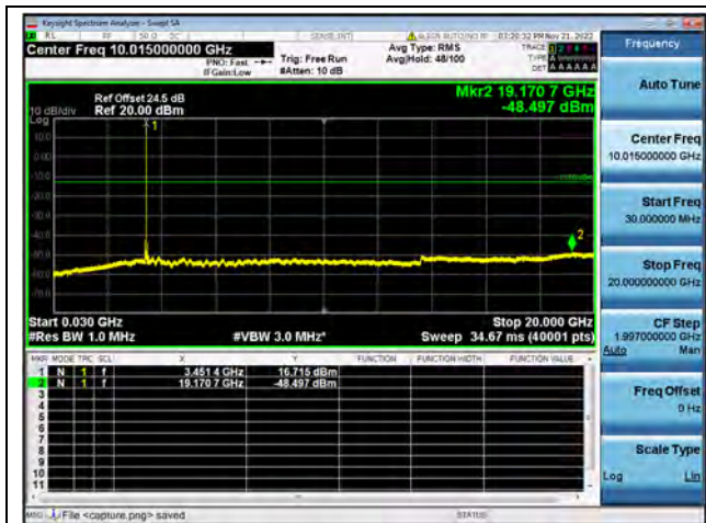
Band42-30M-20G / 15MHz / Low CH / QPSK
