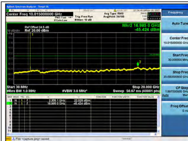
Band30-30M-20G / 10MHz / Mid CH / QPSK
