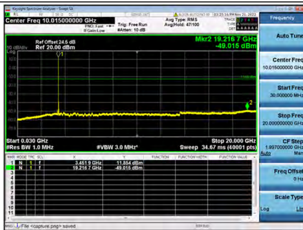
Band42-30M-20G / 20MHz / Low CH / 64QAM
