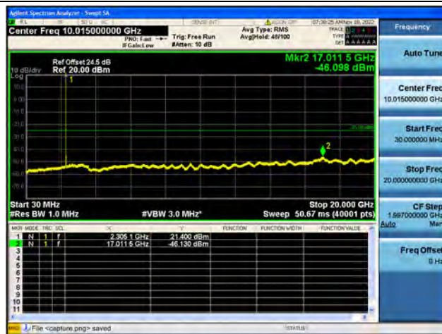
Band30-30M-20G / 10MHz / High CH / 16QAM
