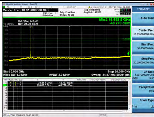
Band42-30M-20G / 20MHz / High CH / 16QAM
