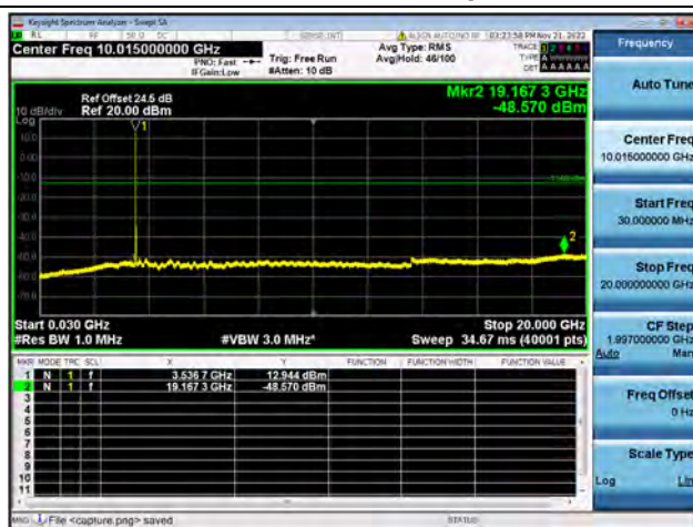
Band42-30M-20G / 15MHz / High CH / 64QAM
