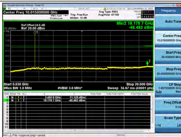
Band42-30M-20G / 5MHz / Low CH / 64QAM
