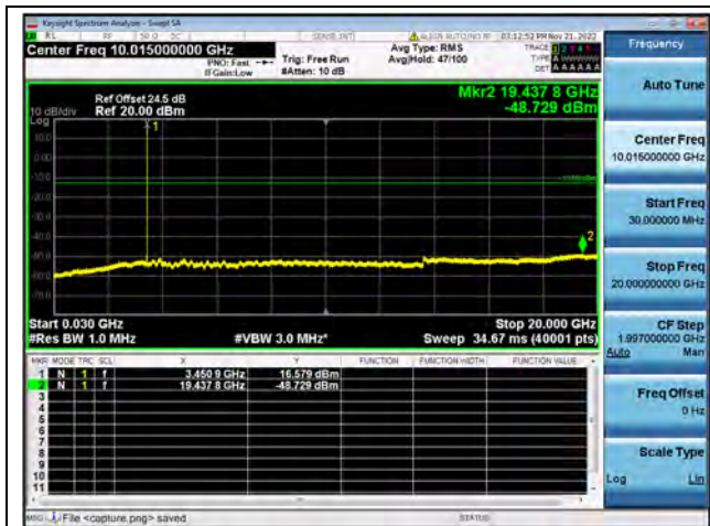
Band42-30M-20G / 5MHz / Low CH / QPSK
