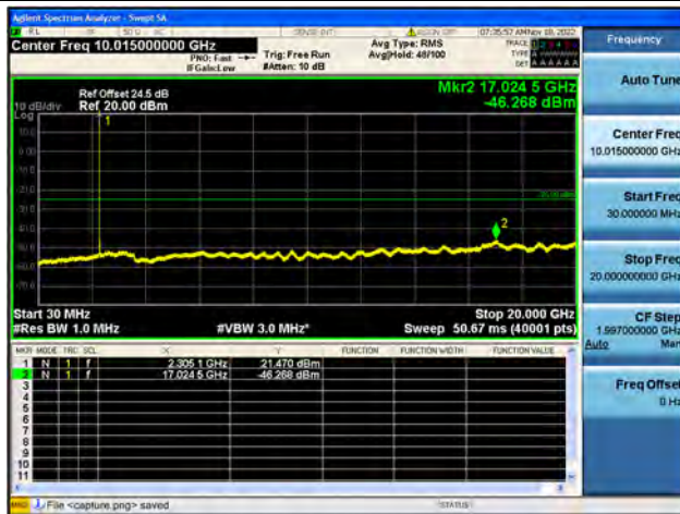
Band30-30M-20G / 10MHz / Low CH / 16QAM
