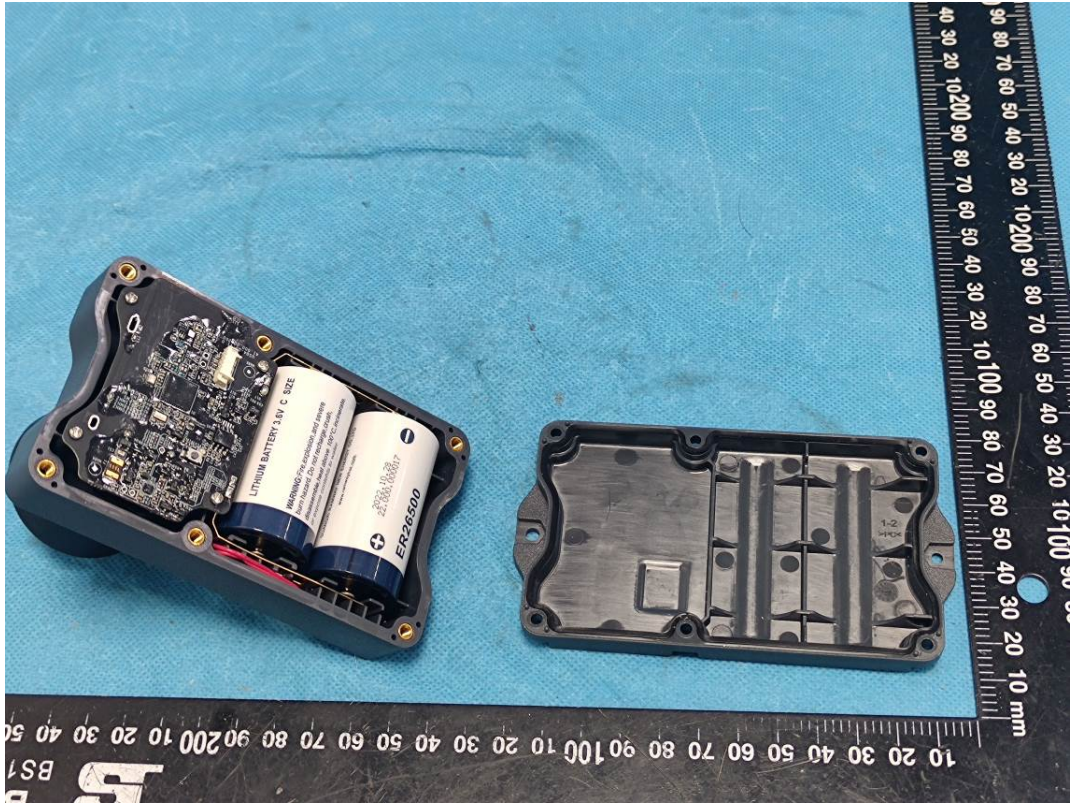
Model: EM400-UDL-915M PN:C050
