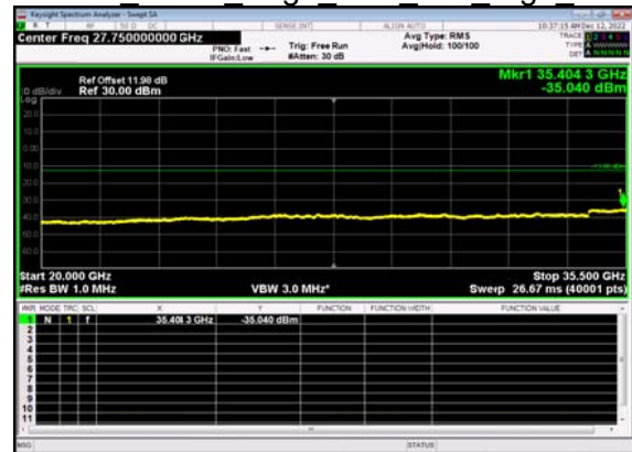
N77(20M)_DFT-s- OFDM BPSK Edge 1RB Left High CH
