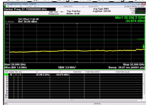
N77(20M)_DFT-s- OFDM QPSK Edge 1RB Left High CH
