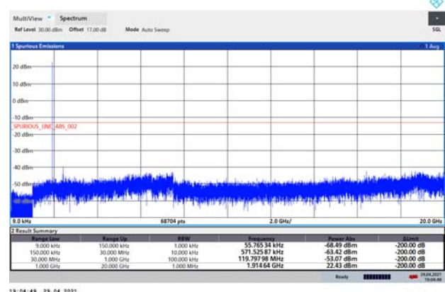
NB-IoT Band 25 CH-High 9kHz~20GHz
