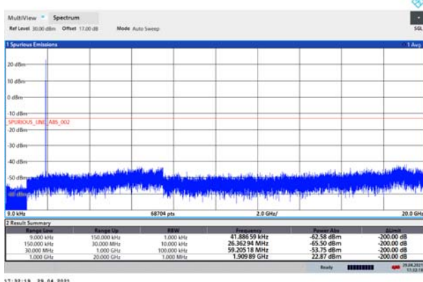
NB-IoT Band 2 CH-High 9kHz~20GHz
