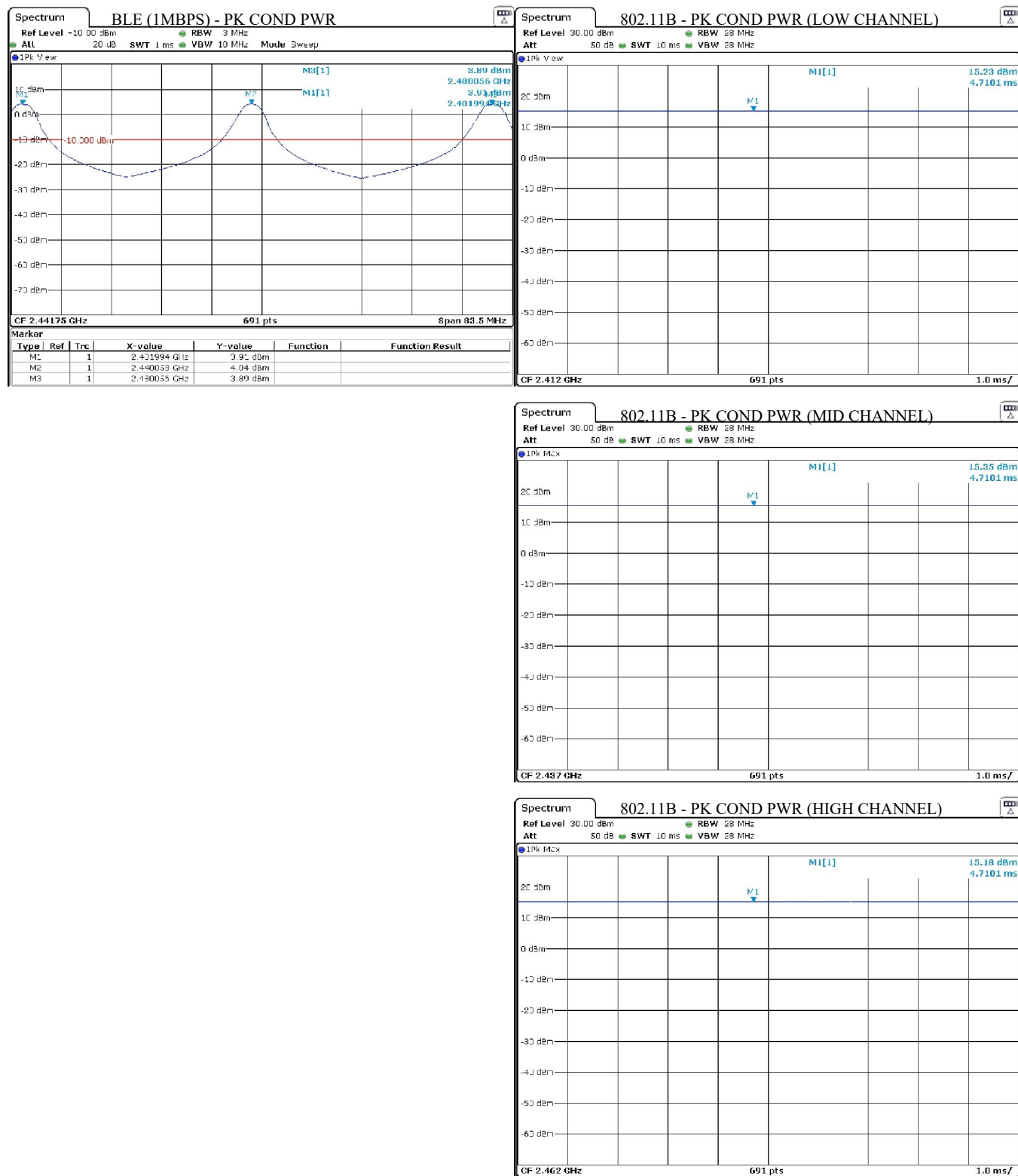
Figure 8(a): Conducted RF Power Plots
