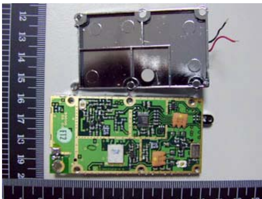
Photo 6: Handset inner
