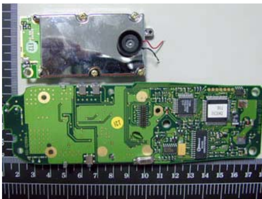
Photo 5: Handset inner
