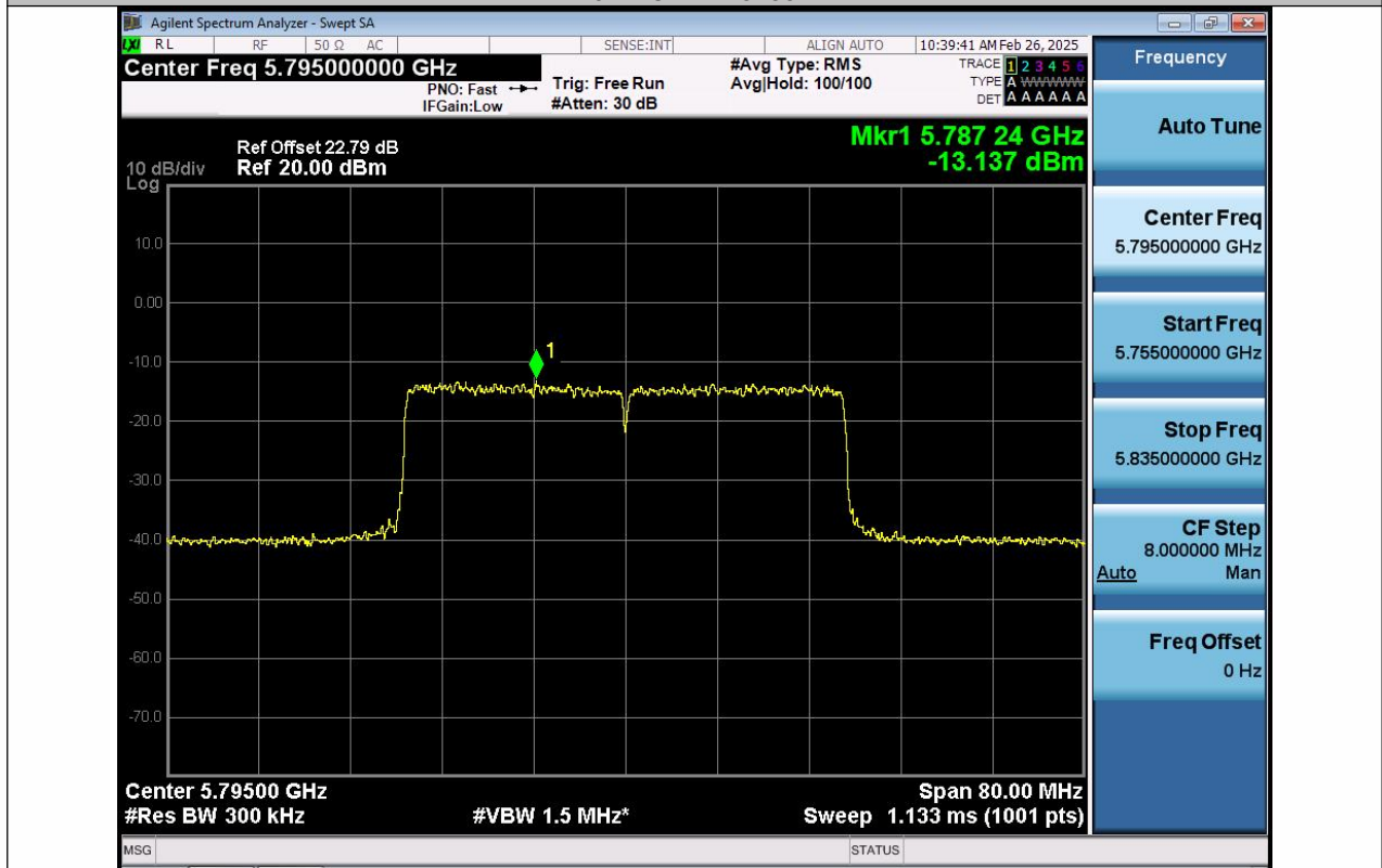
11AX40SISO-Ant1-5795-PASS
