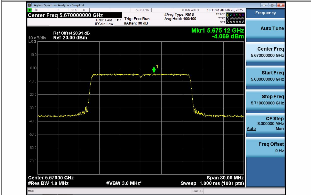
11AX40SISO-Ant1-5670-PASS
