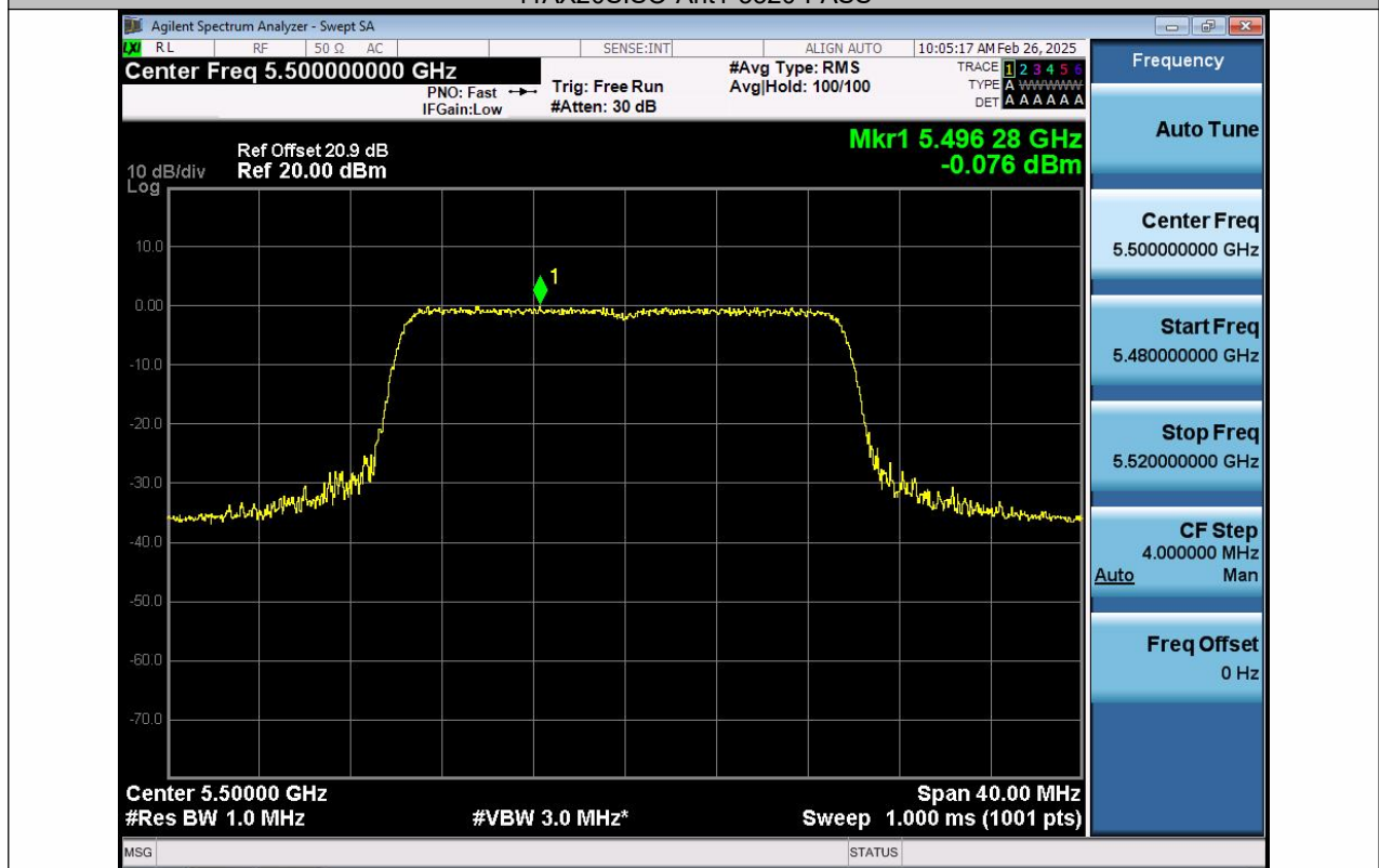
11AX20SISO-Ant1-5500-PASS
