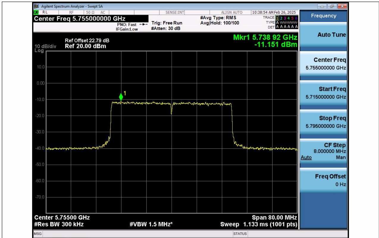
11AX40SISO-Ant1-5755-PASS
