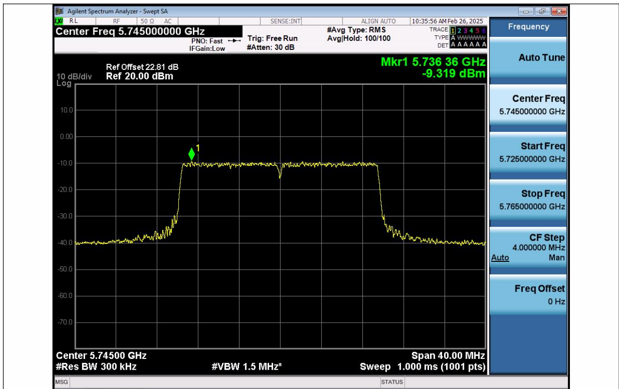
11AX20SISO-Ant1-5745-PASS
