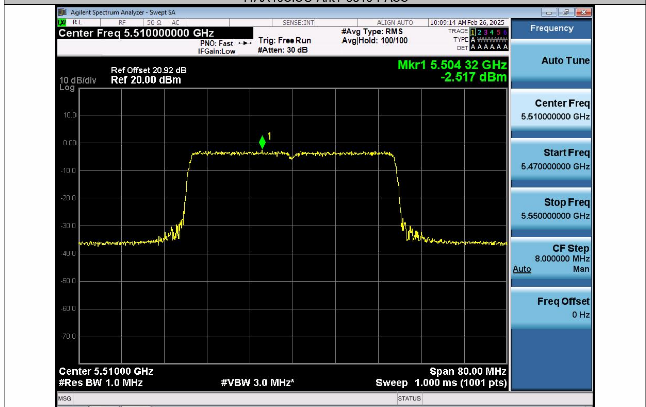
11AX40SISO-Ant1-5510-PASS
