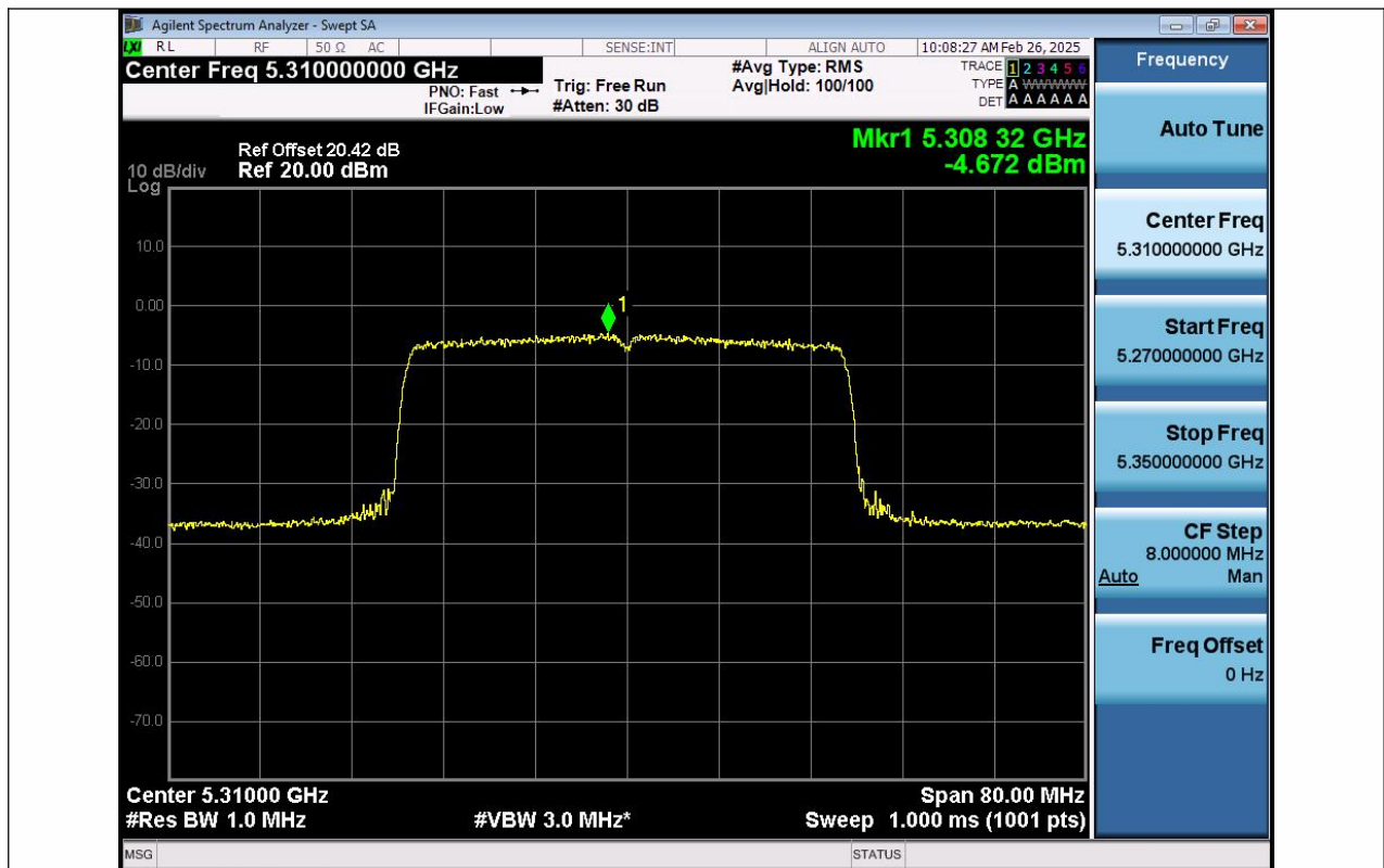
11AX40SISO-Ant1-5310-PASS
