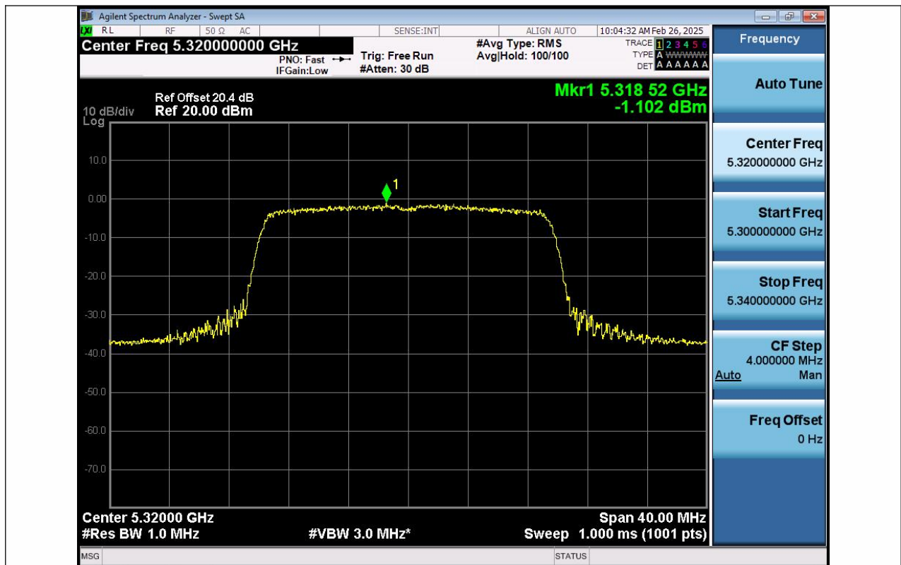
11AX20SISO-Ant1-5320-PASS
