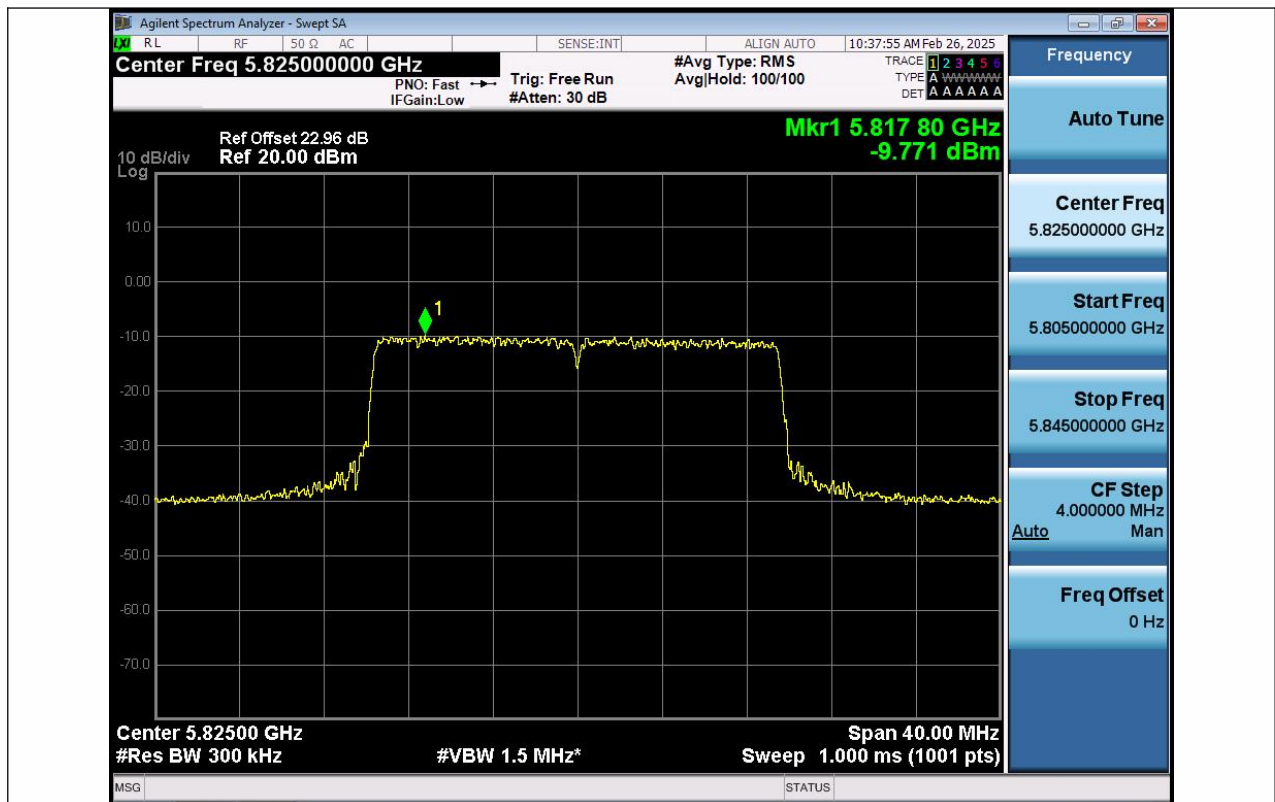
11AX20SISO-Ant1-5825-PASS
