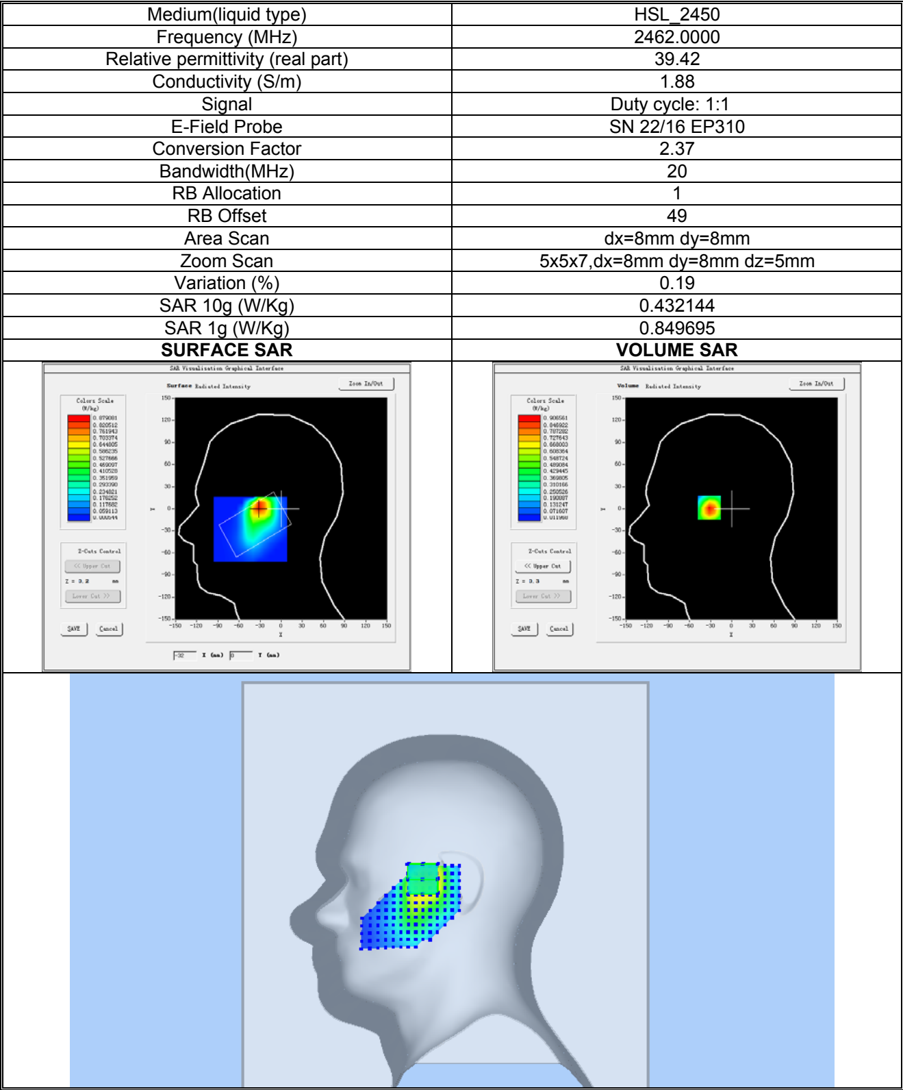
Plot 13:802.11b, High channel (Right Head Cheek) Product Description: CELLPHONE Test Date: 2022-04-11
