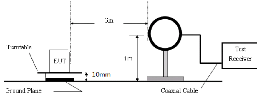
Figure1. Below 30MHz radiated emissions test configuration
