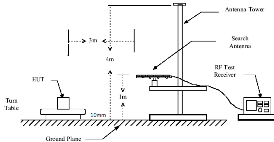
Figure 2. 30MHz to 1GHz radiated emissions test configuration
