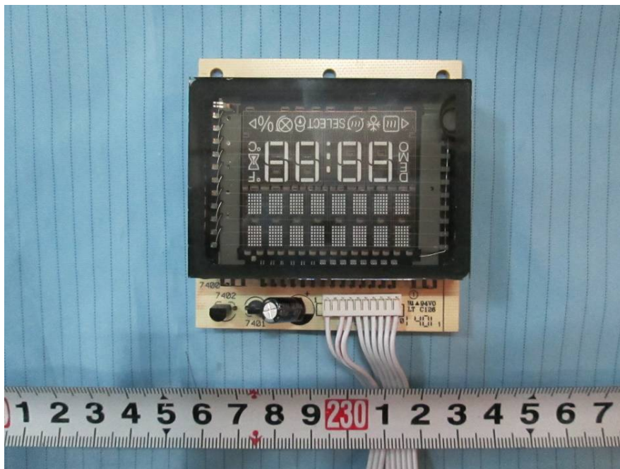
EUT – LED PCB Board Top View
