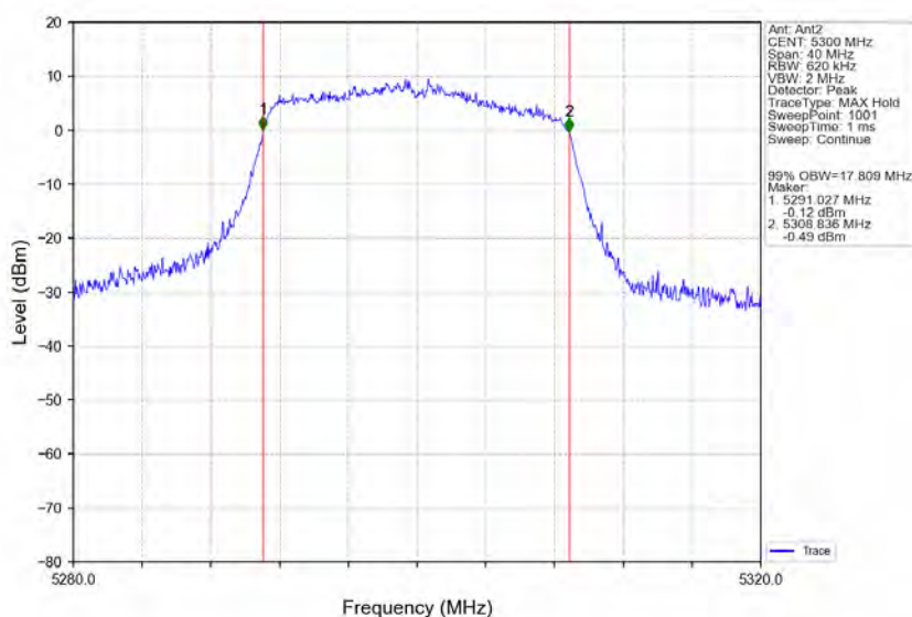
802.11ac(VHT20)_MCH_5300MHz_Ant2_NTNV
