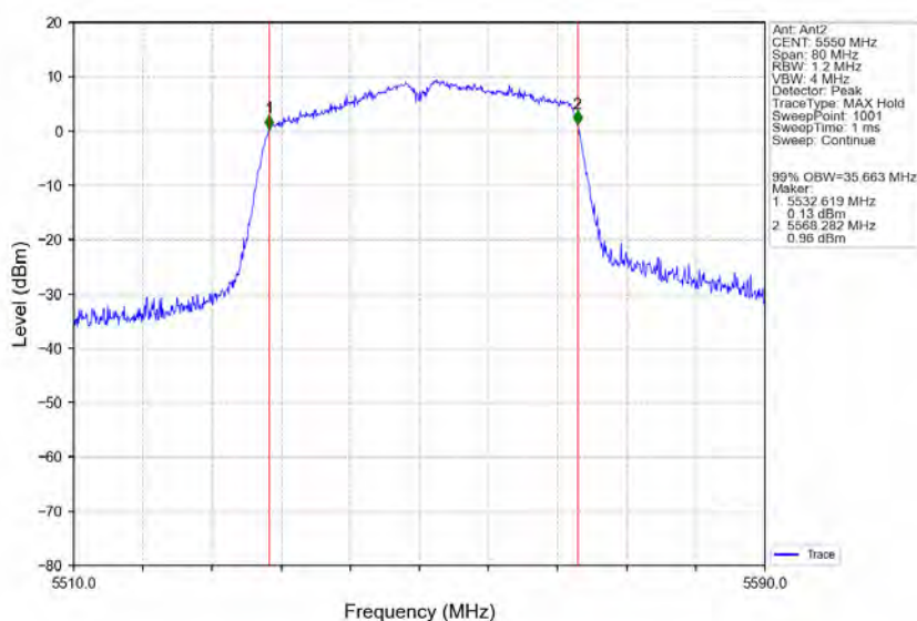
802.11ac(VHT40)_MCH_5550MHz_Ant2_NTNV
