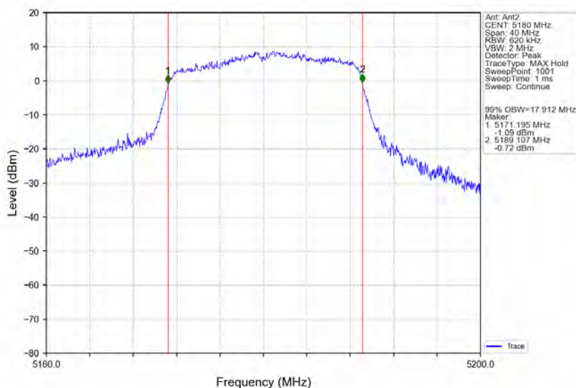
802.11ac(VHT20) LCH_5180MHz_Ant2_NTNV
