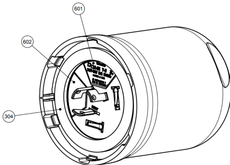
Figure 1 Assembly drawing showing the location of the T2A4N labels
